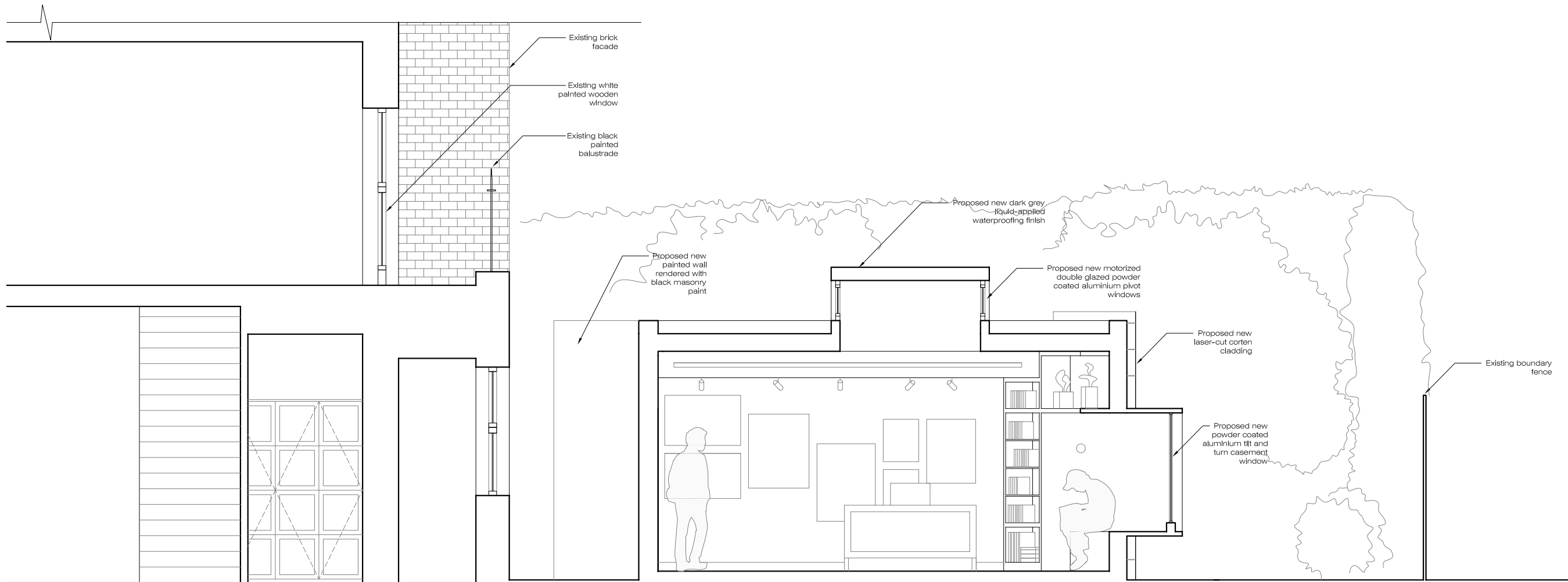
01 Proposed Section CC' scale: 1:50
