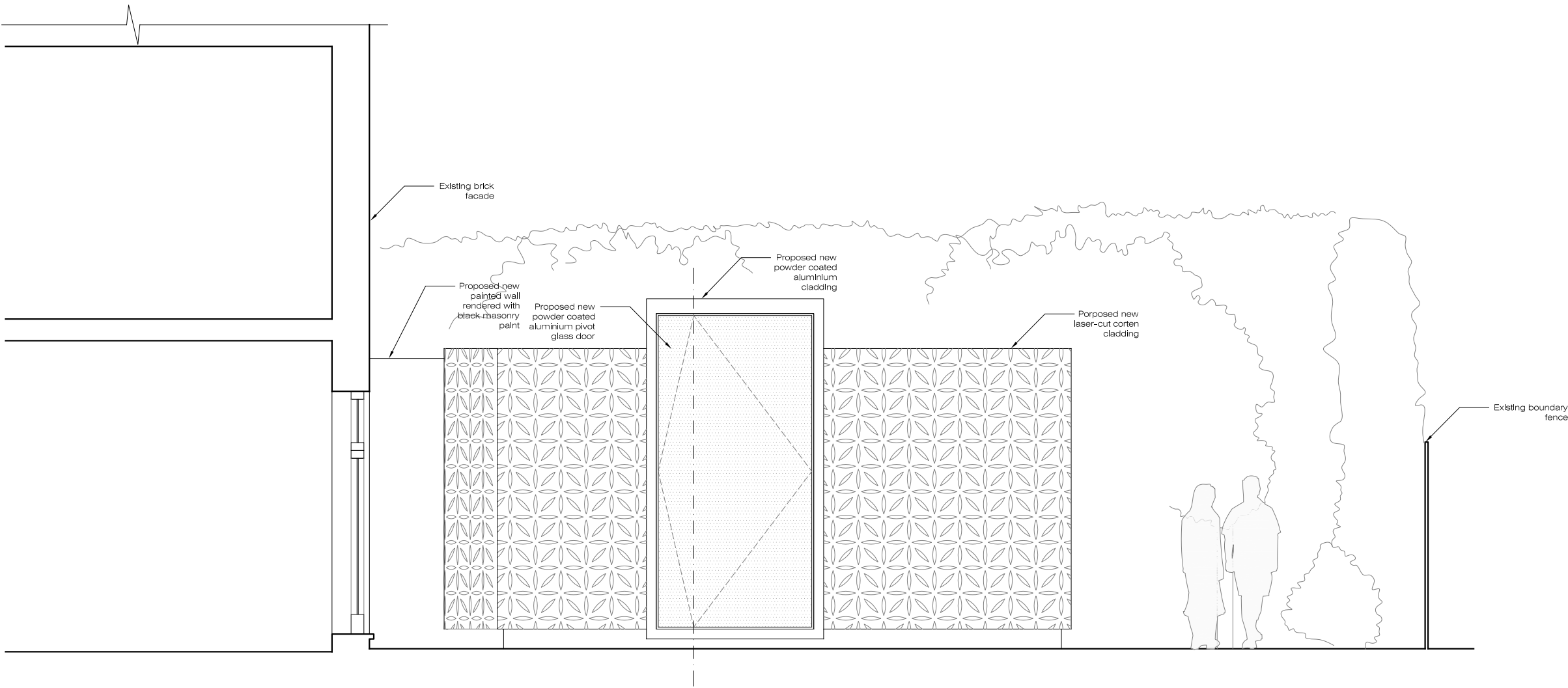
01 Proposed Elevation AA' scale: 1:50
