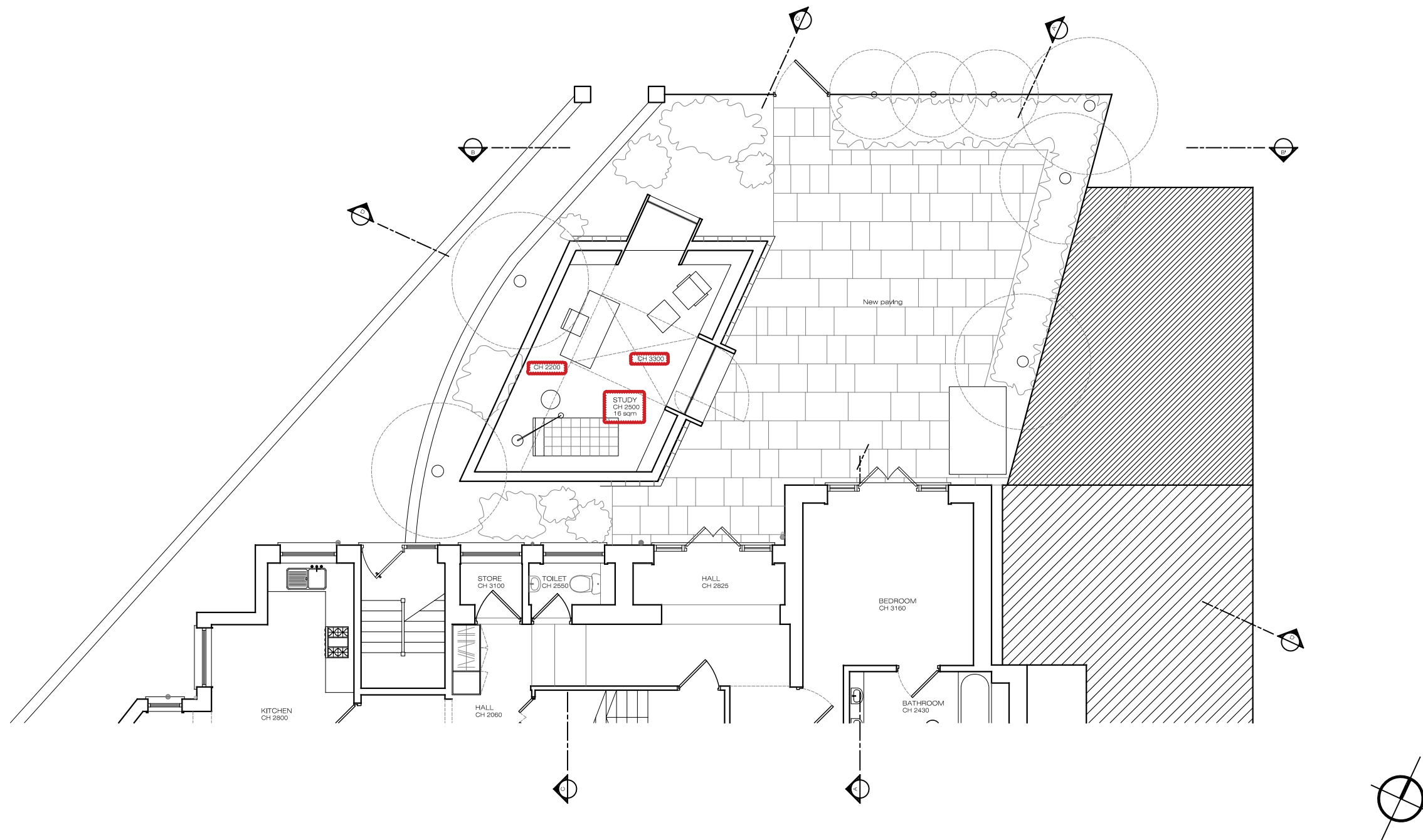
01 Proposed Ground Floor scale: 1:100
