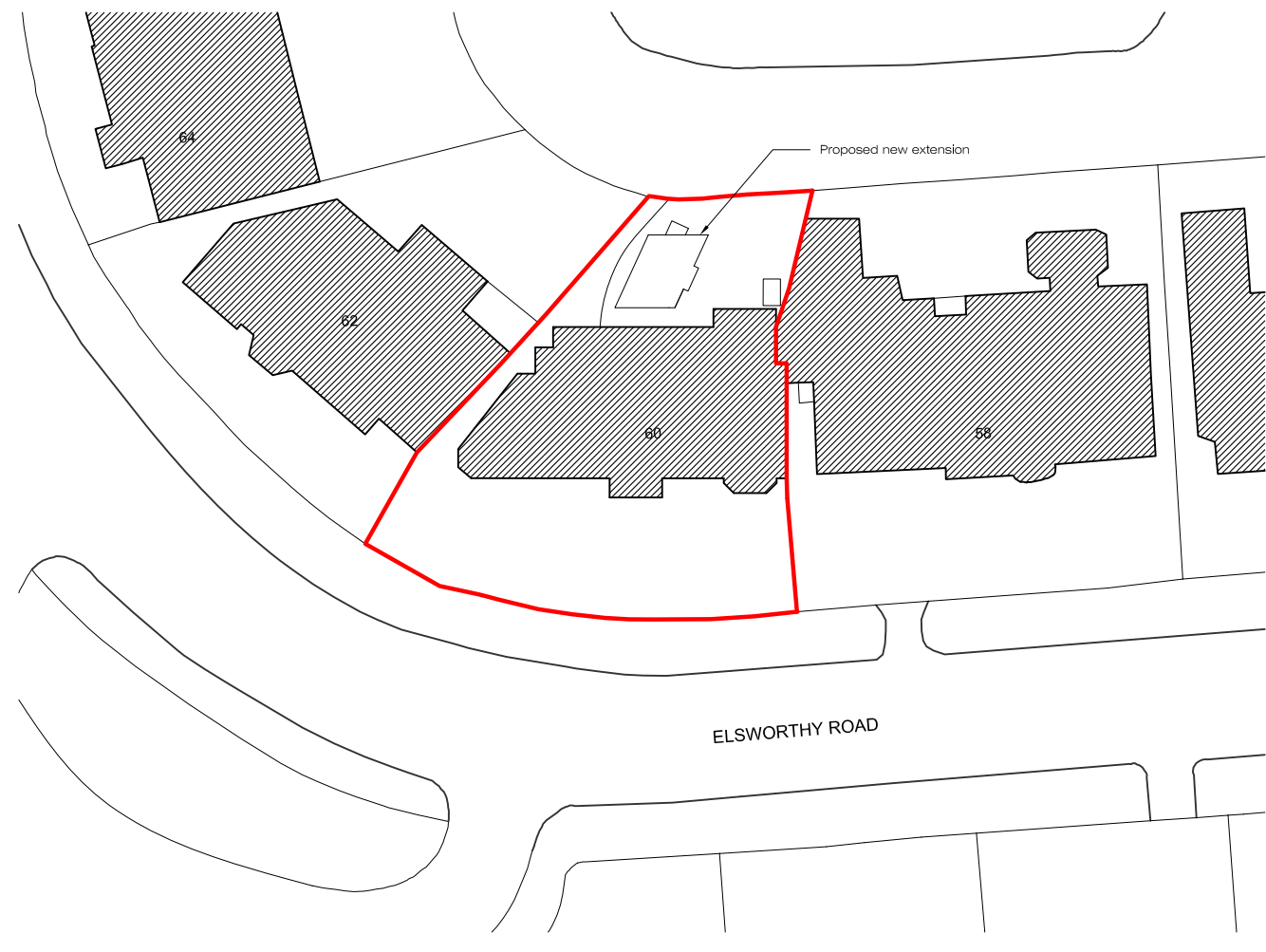
01 Proposed Site Plan scale: 1:500
