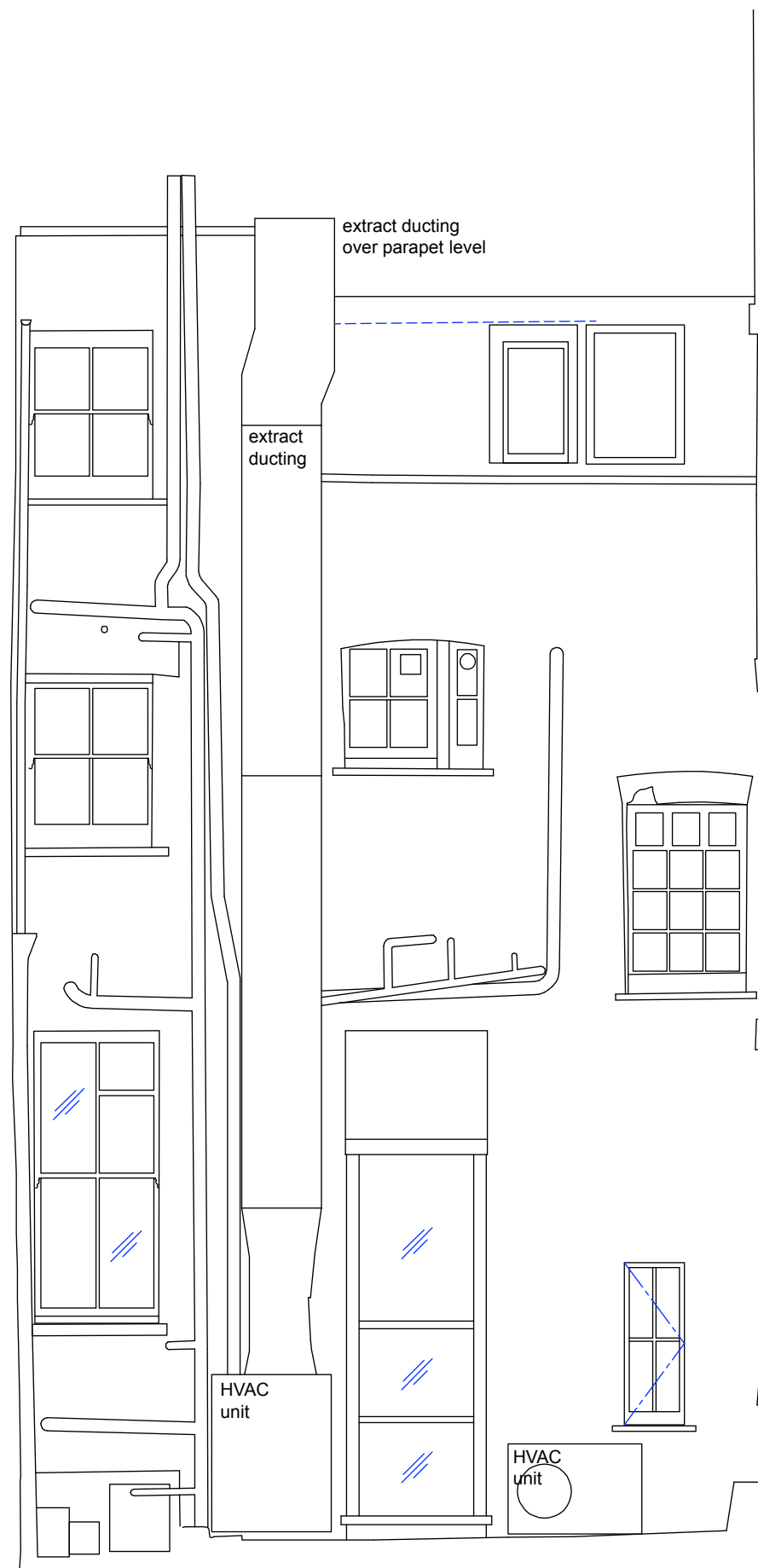
7 Existing Rear Elevation 1:50@A3
