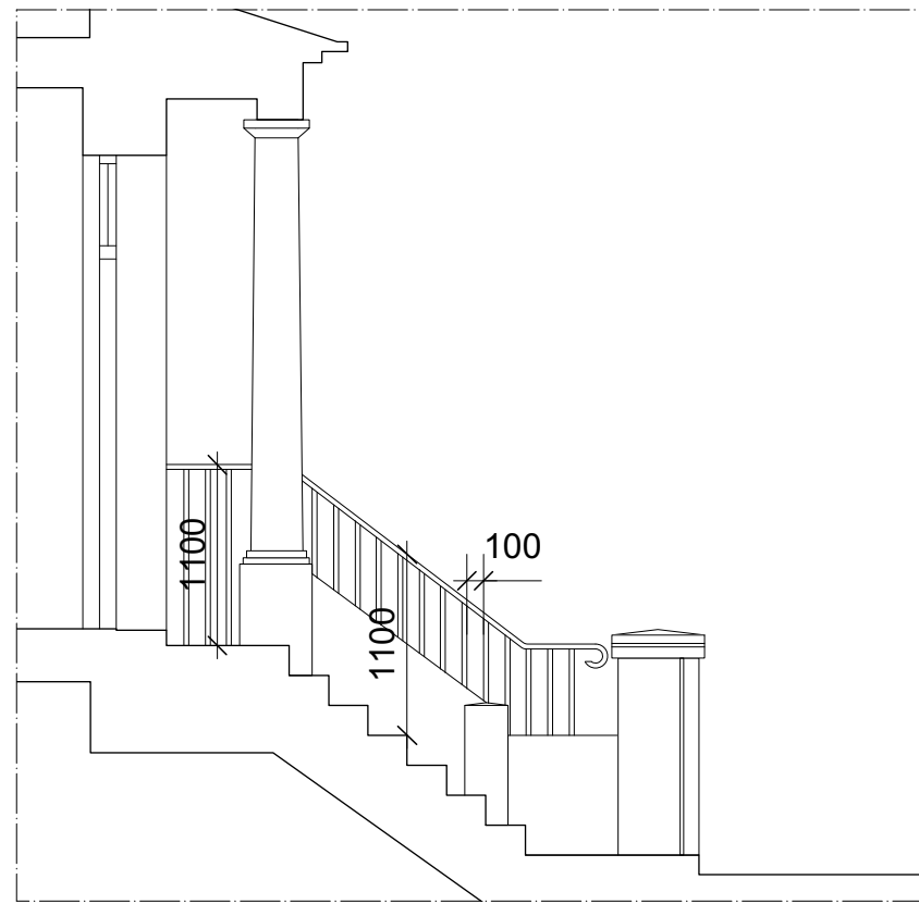
○ PROPOSED HANDRAIL Scale 1:50
