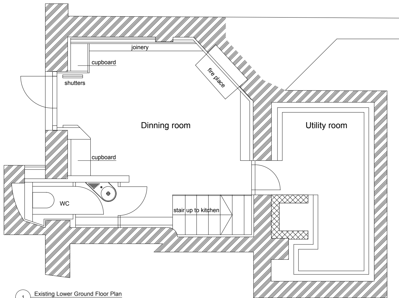
1 Existing Lower Ground Floor Plan
