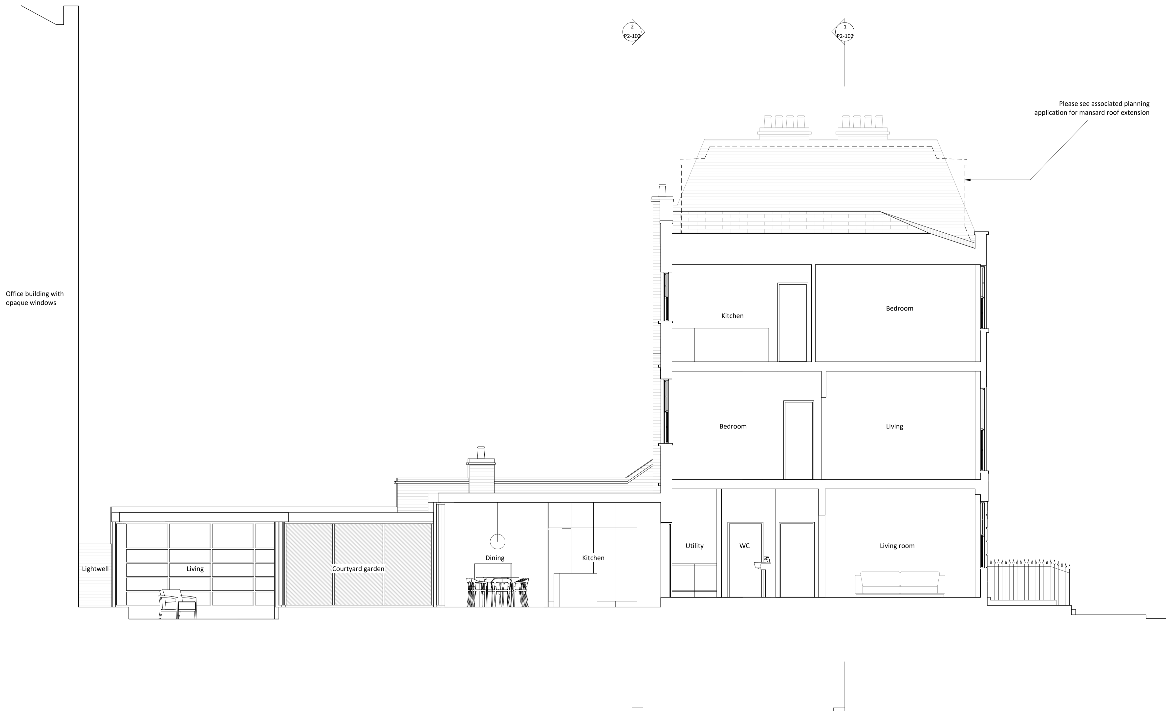
Section 2 1:50
