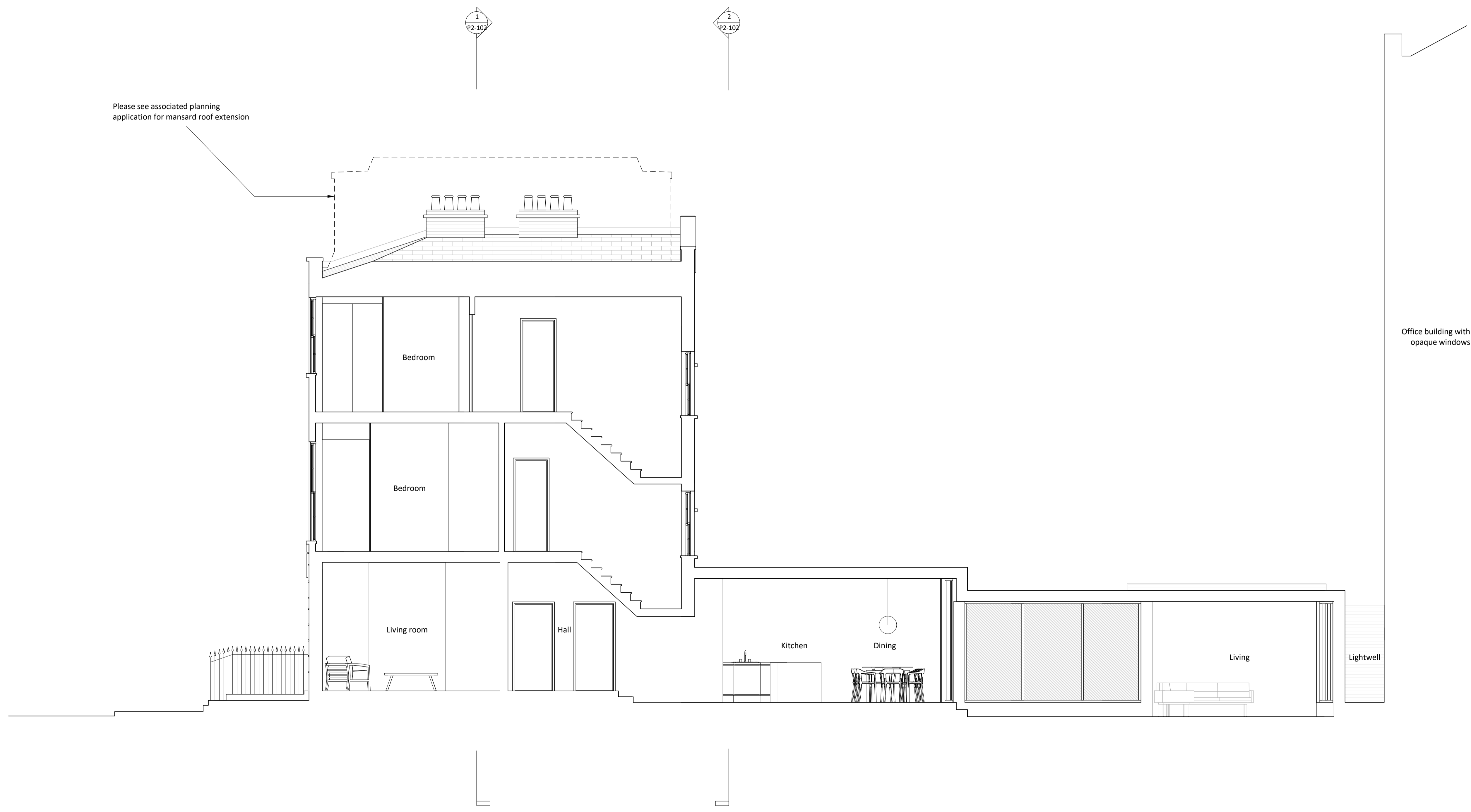
Section 1 1:50
