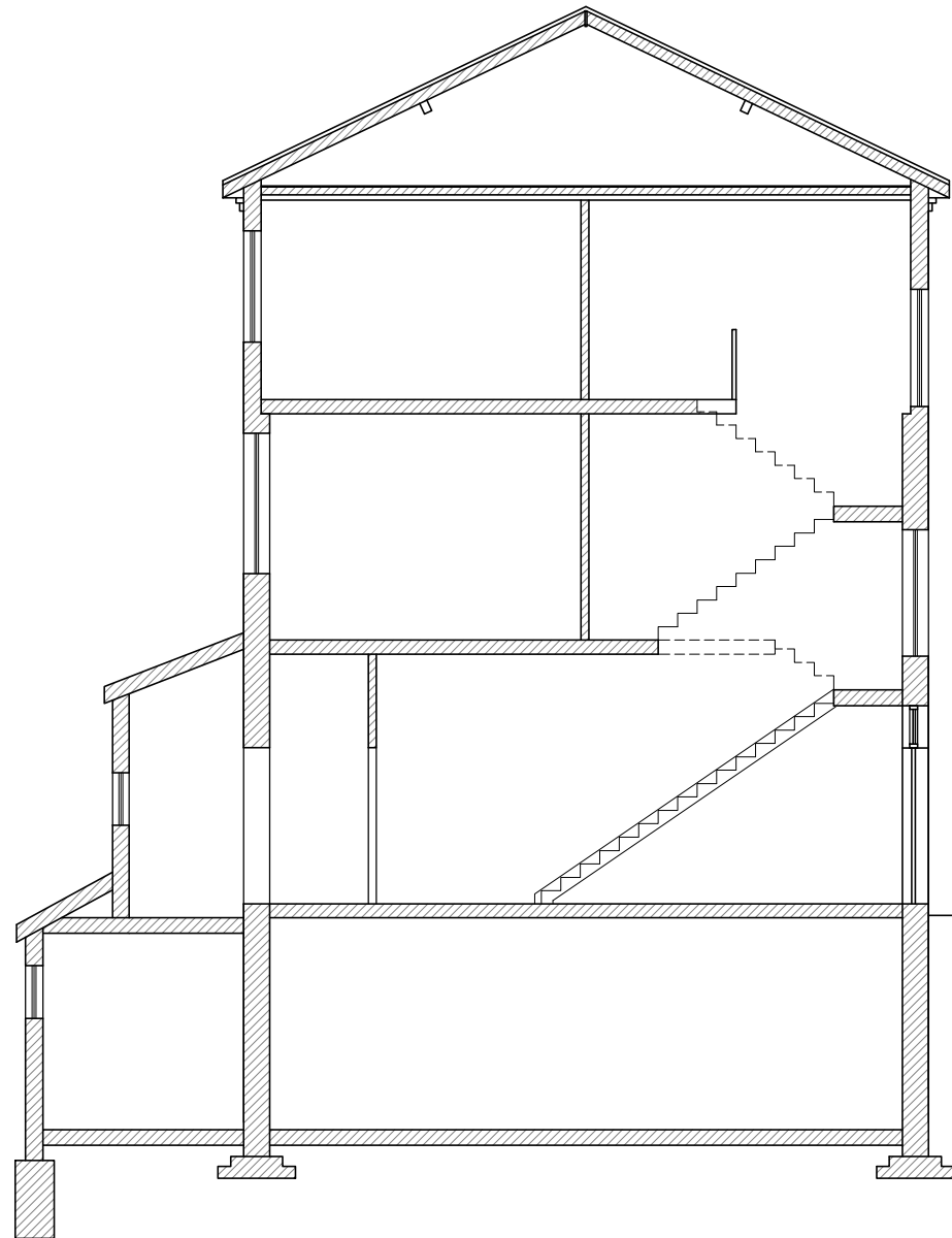
SECTION B-B
