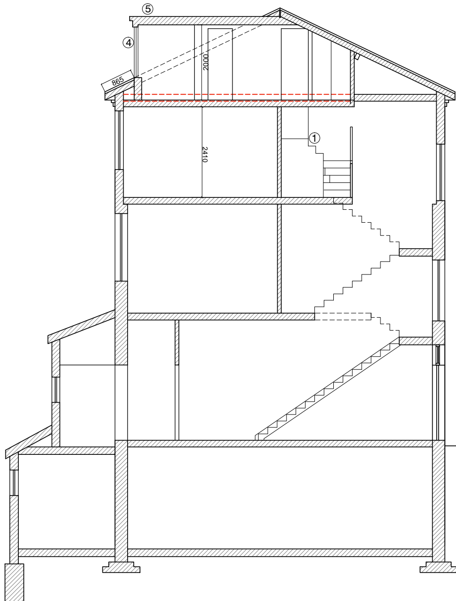
SECTION B-B
