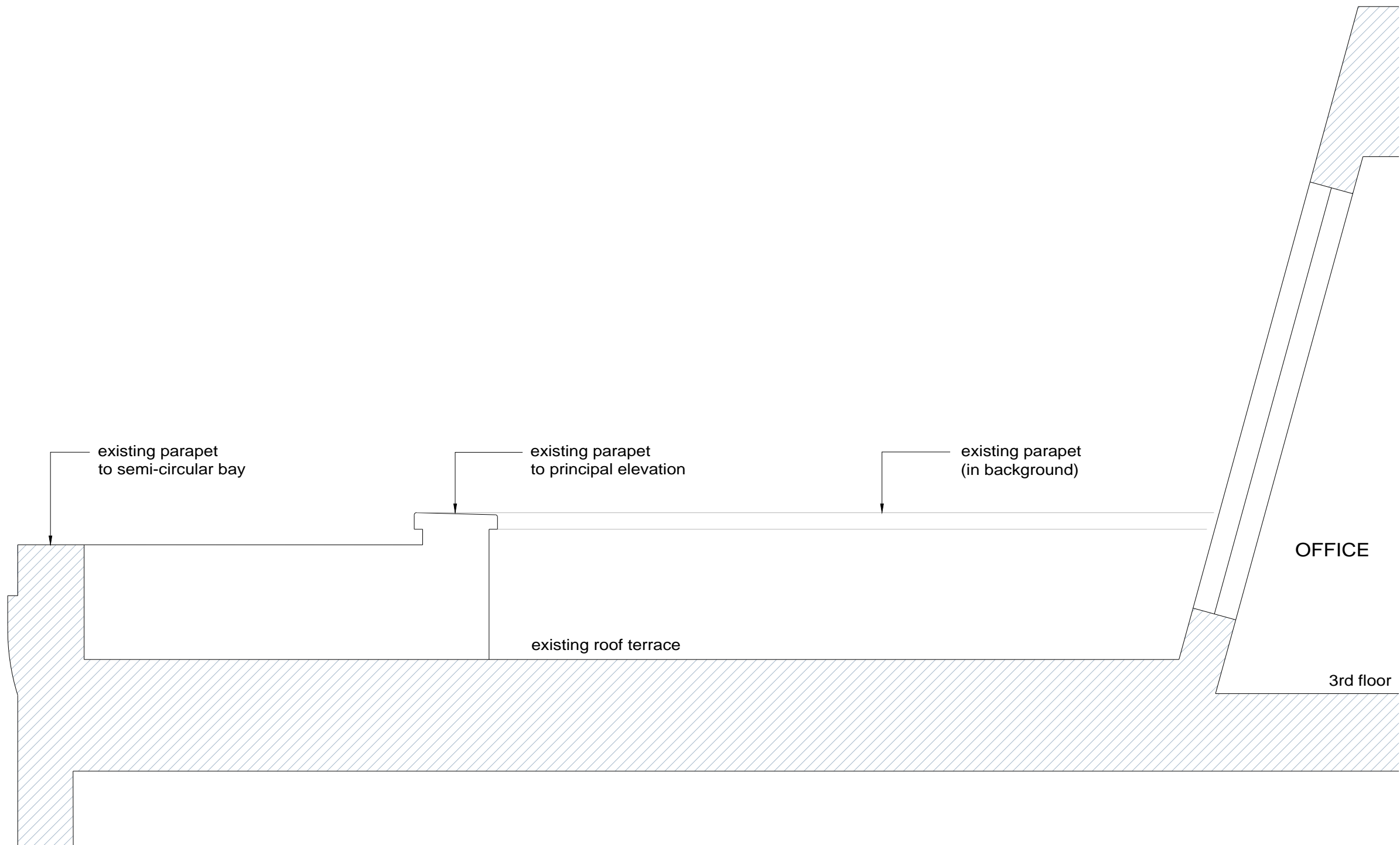
DETAIL SECTION B-B 1:20 @ A3
