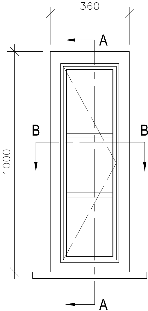
Internal Elevation
