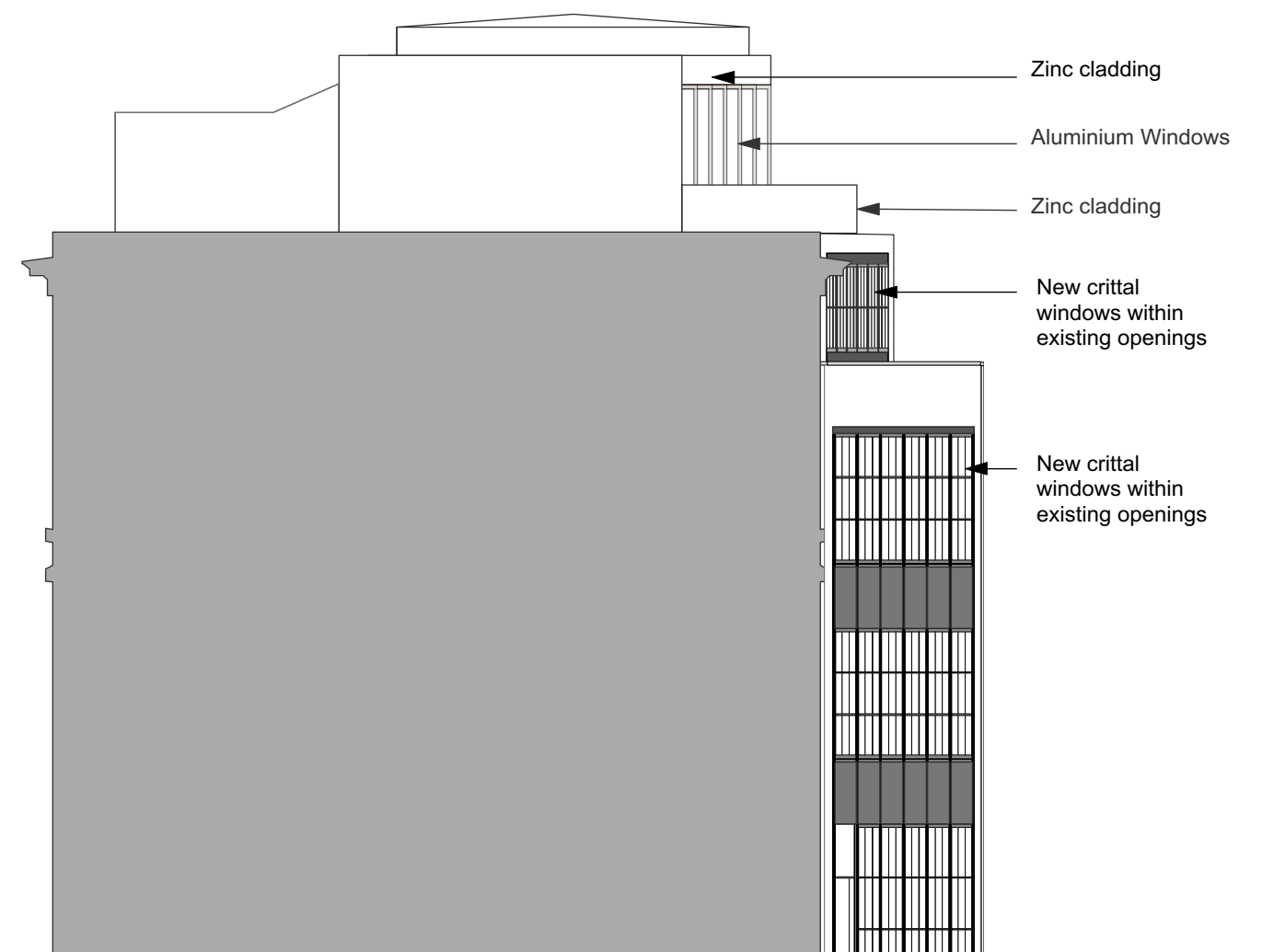
5 Section C-C- Proposed Scale: 1:100
