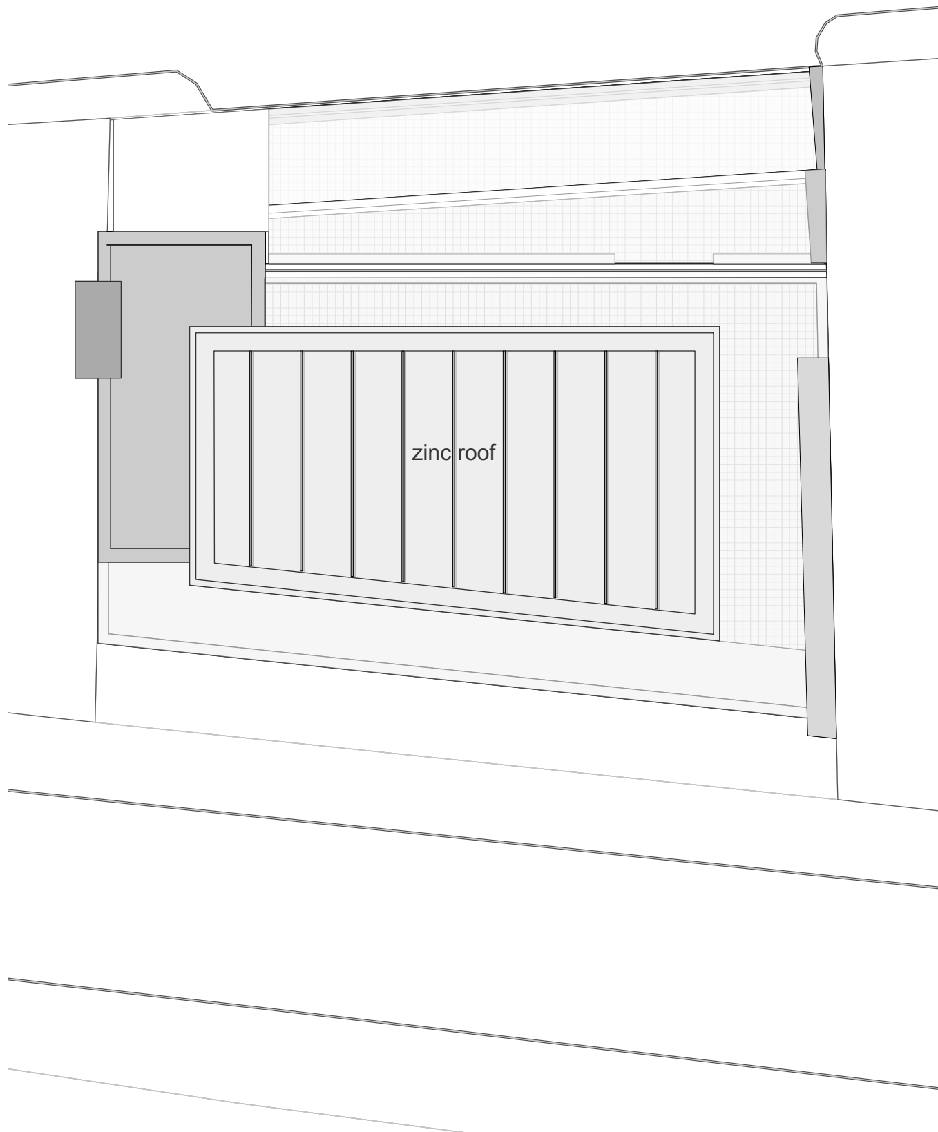
1 Roof Plan - Proposed Scale: 1:100
