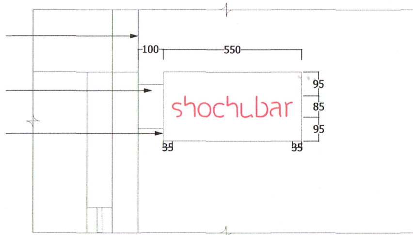
03 ROKA Charlotte Street - Proposed Side Elevation BB SCALE 1:5 @ A1
