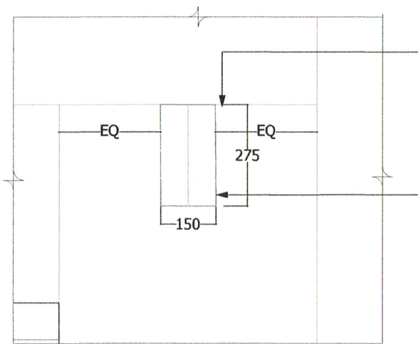
02 ROKA Charlotte Street - Proposed Front Elevation AA SCALE 1:5 @ A1
