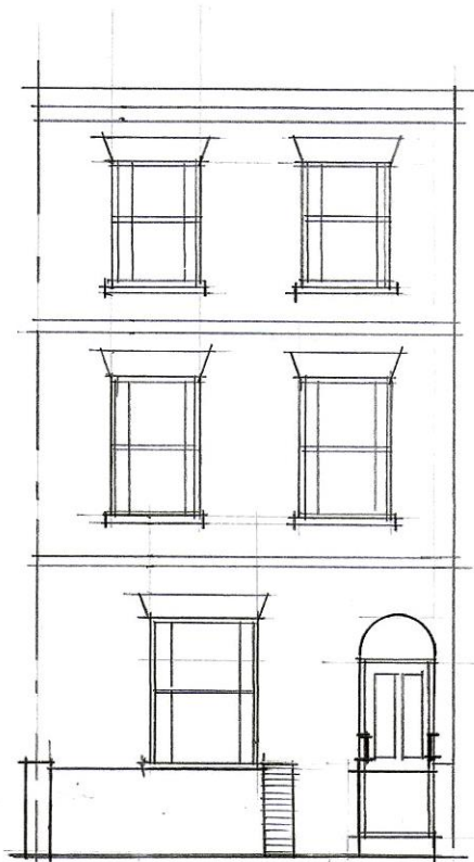
FRONT ELEVATION 1:100
