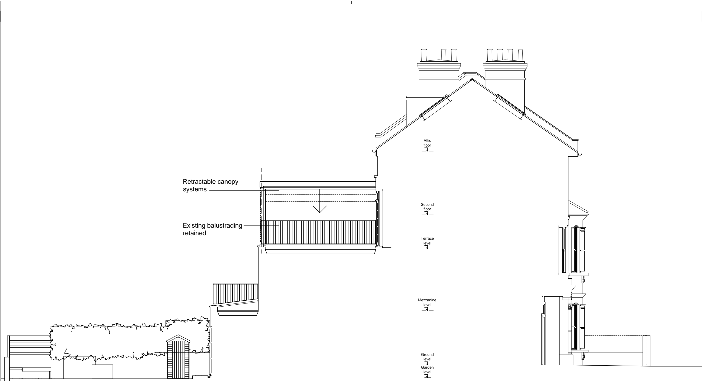
01 - LONG SECTION - PROPOSED
