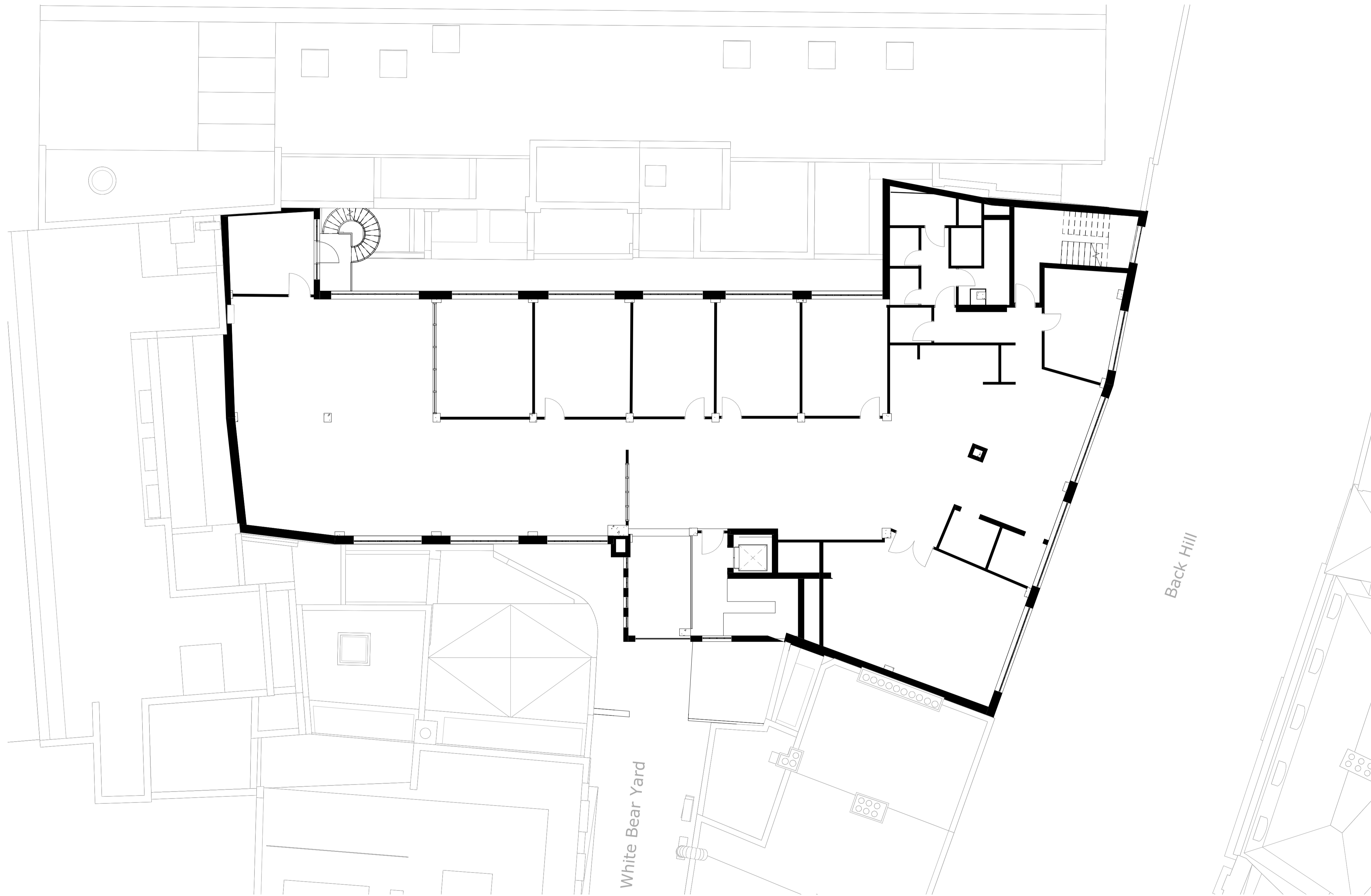
01 Existing First Floor Plan 1 : 100
