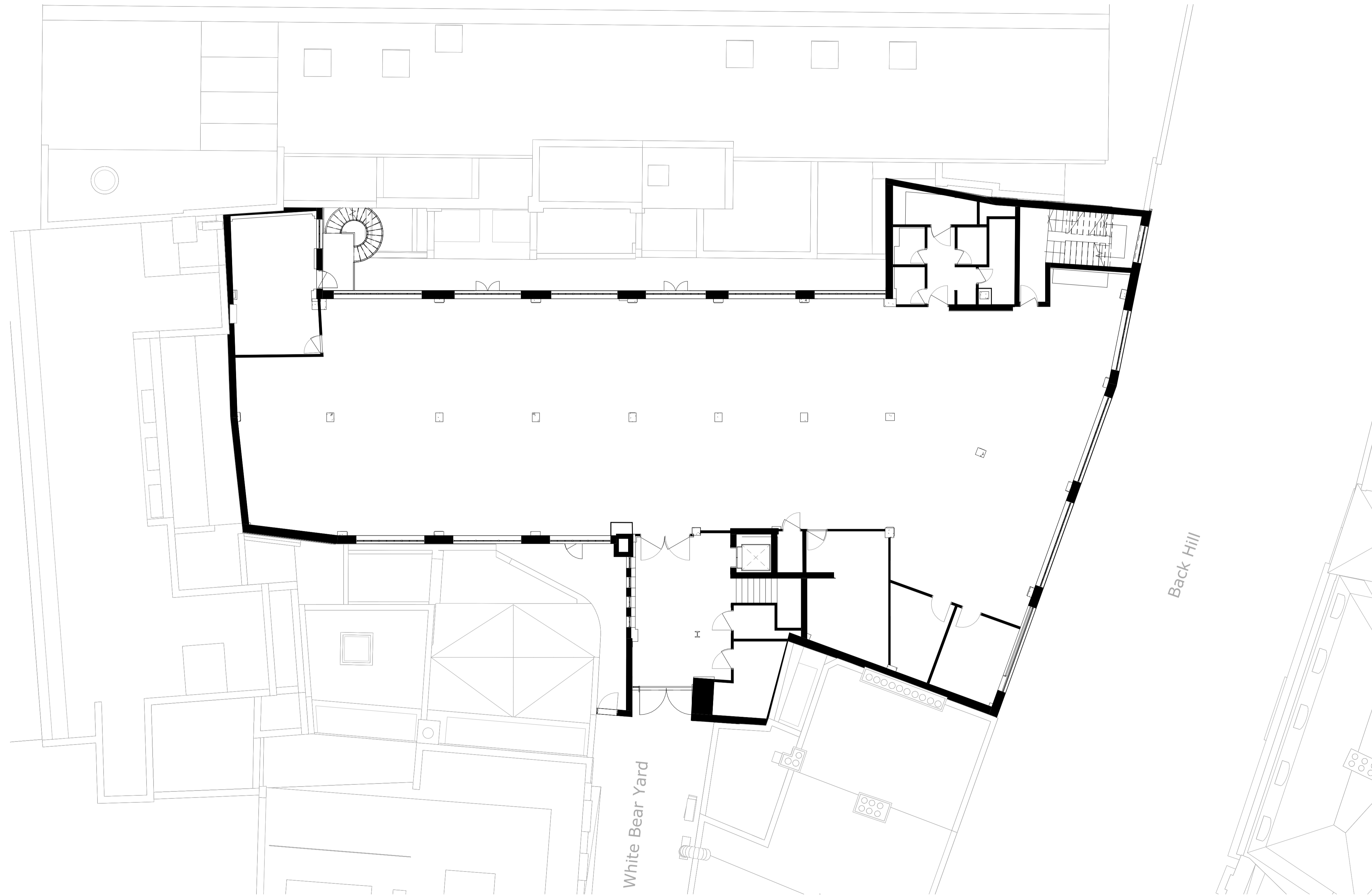
00 Existing Ground Floor Plan 1 : 100
