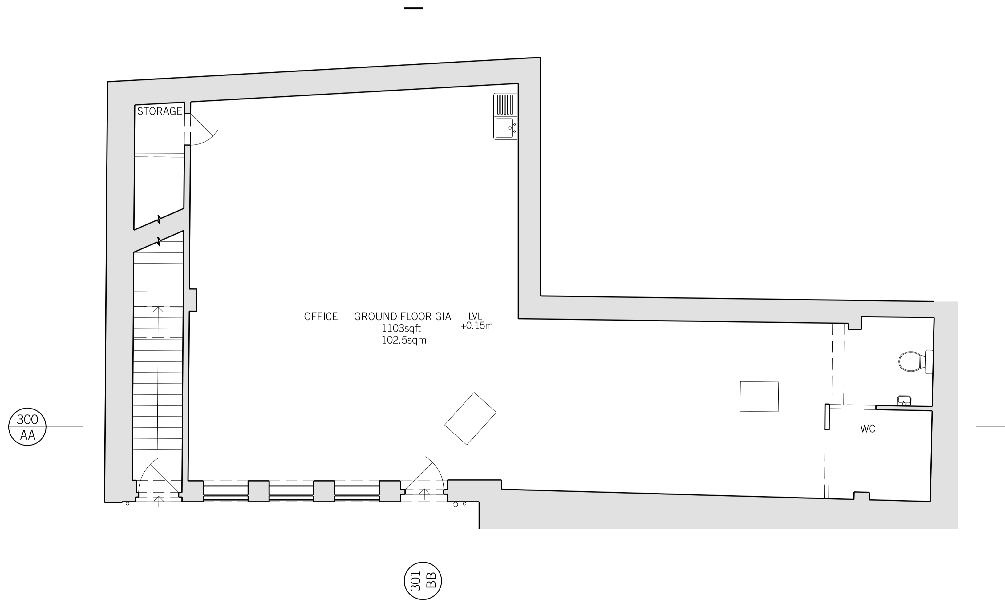
01: EXISTING GROUND FLOOR PLAN SCALE 1:50
