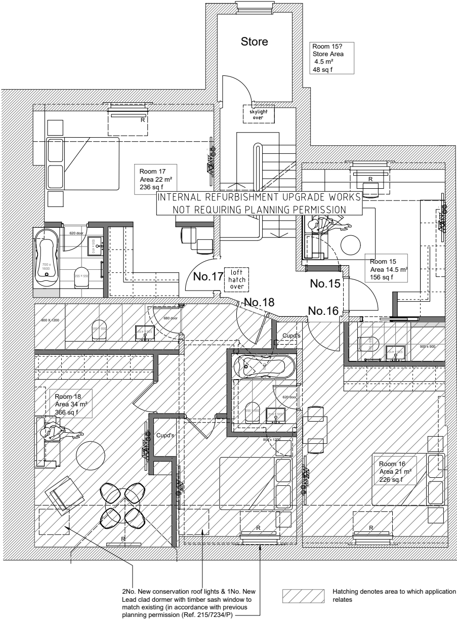
THIRD FLOOR PLAN (PROPOSED)
