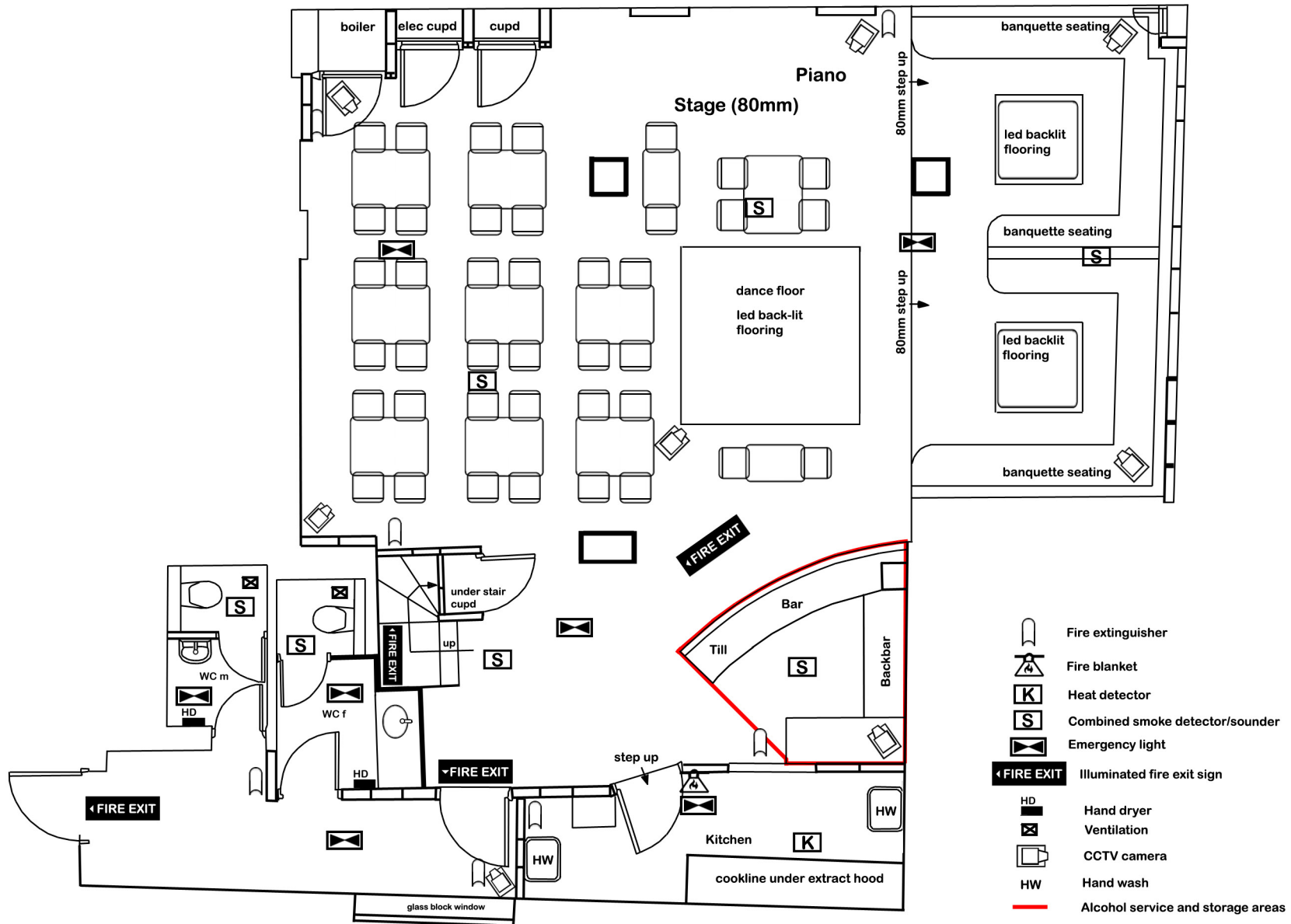
Basement plan
