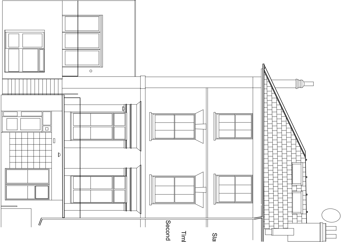
REAR ELEVATION AS EXISTING
