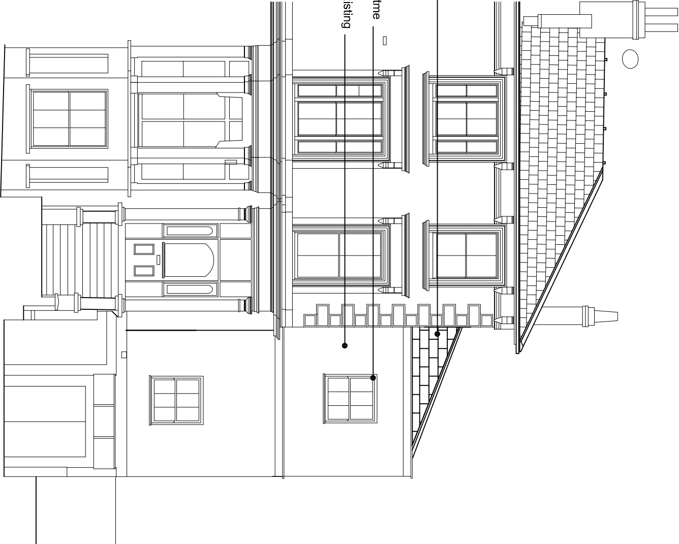
FRONT ELEVATION AS PROPOSED
