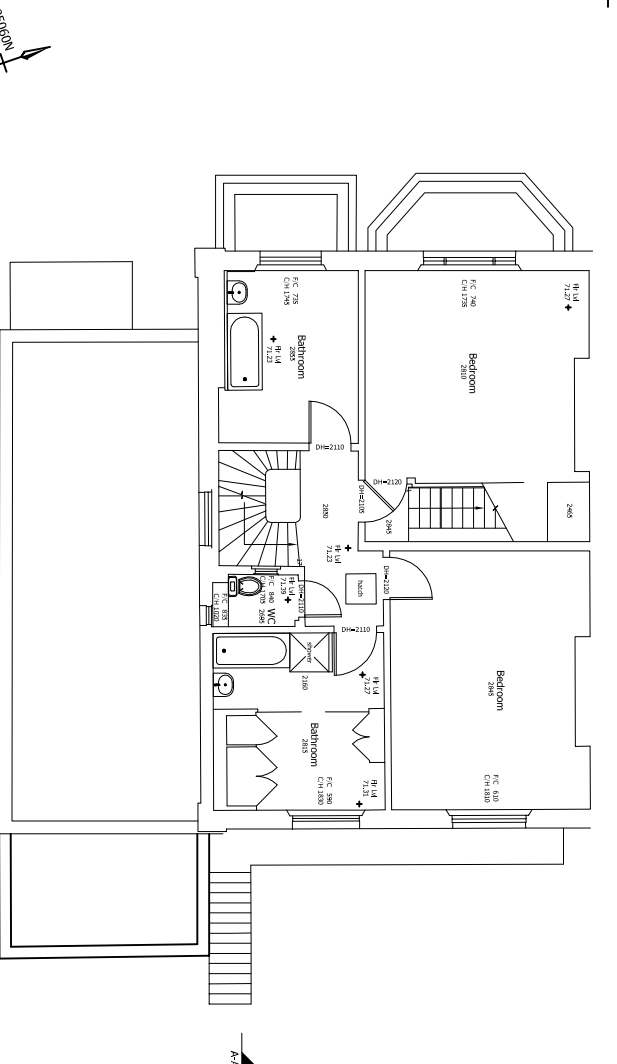
THIRD FLOOR PLAN AS EXISTING
