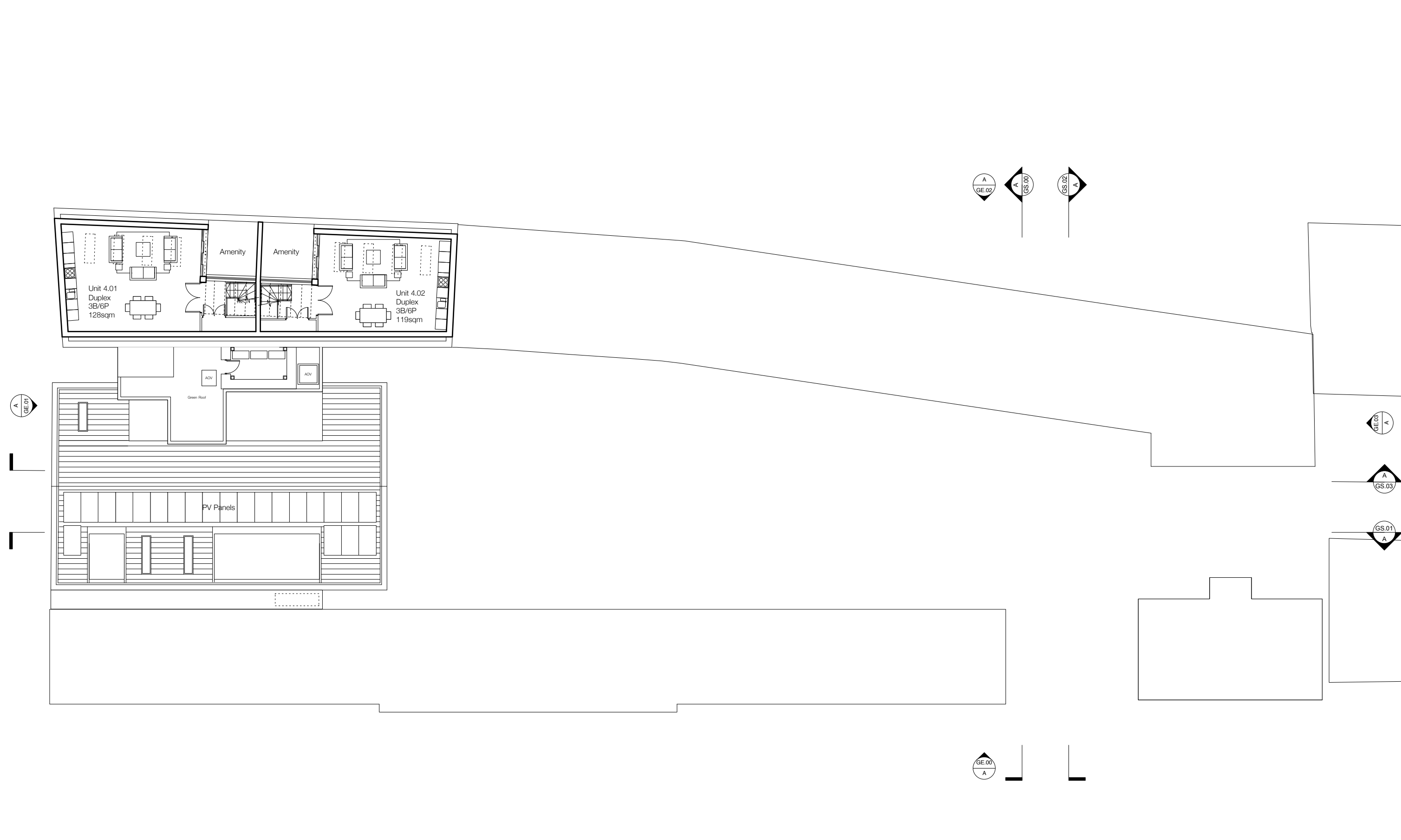
A Proposed Fifth Floor General arrangement GA.05 1:100 @A1 1:200 @A3
