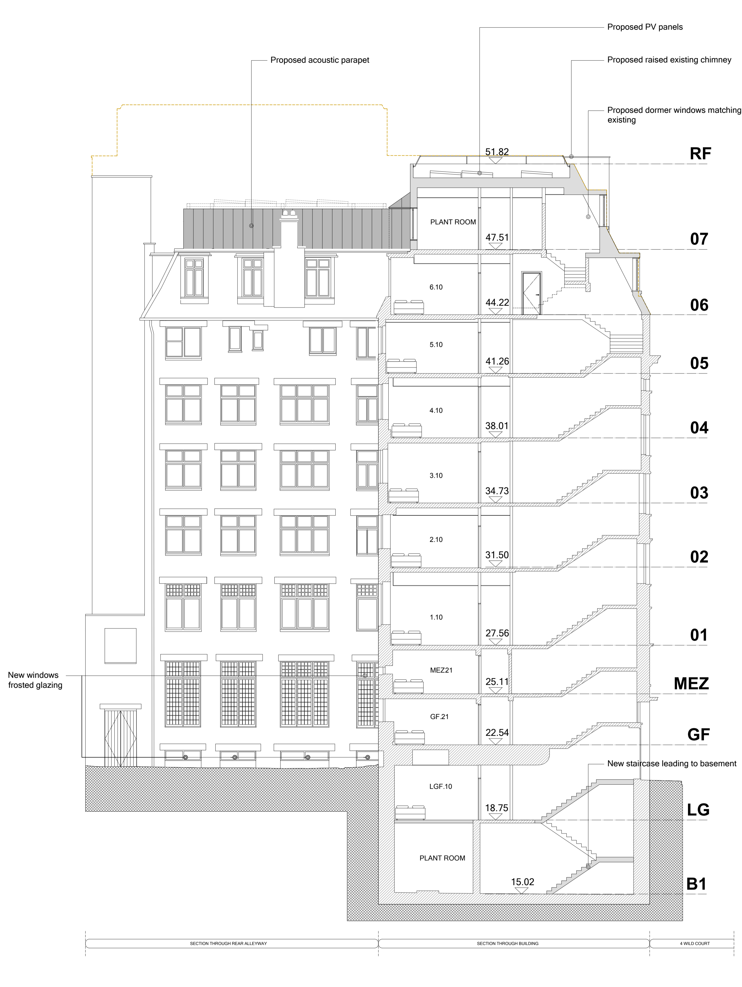
02 Proposed Elevation 04 ( Wild Court Elevation) Scale 1/100
