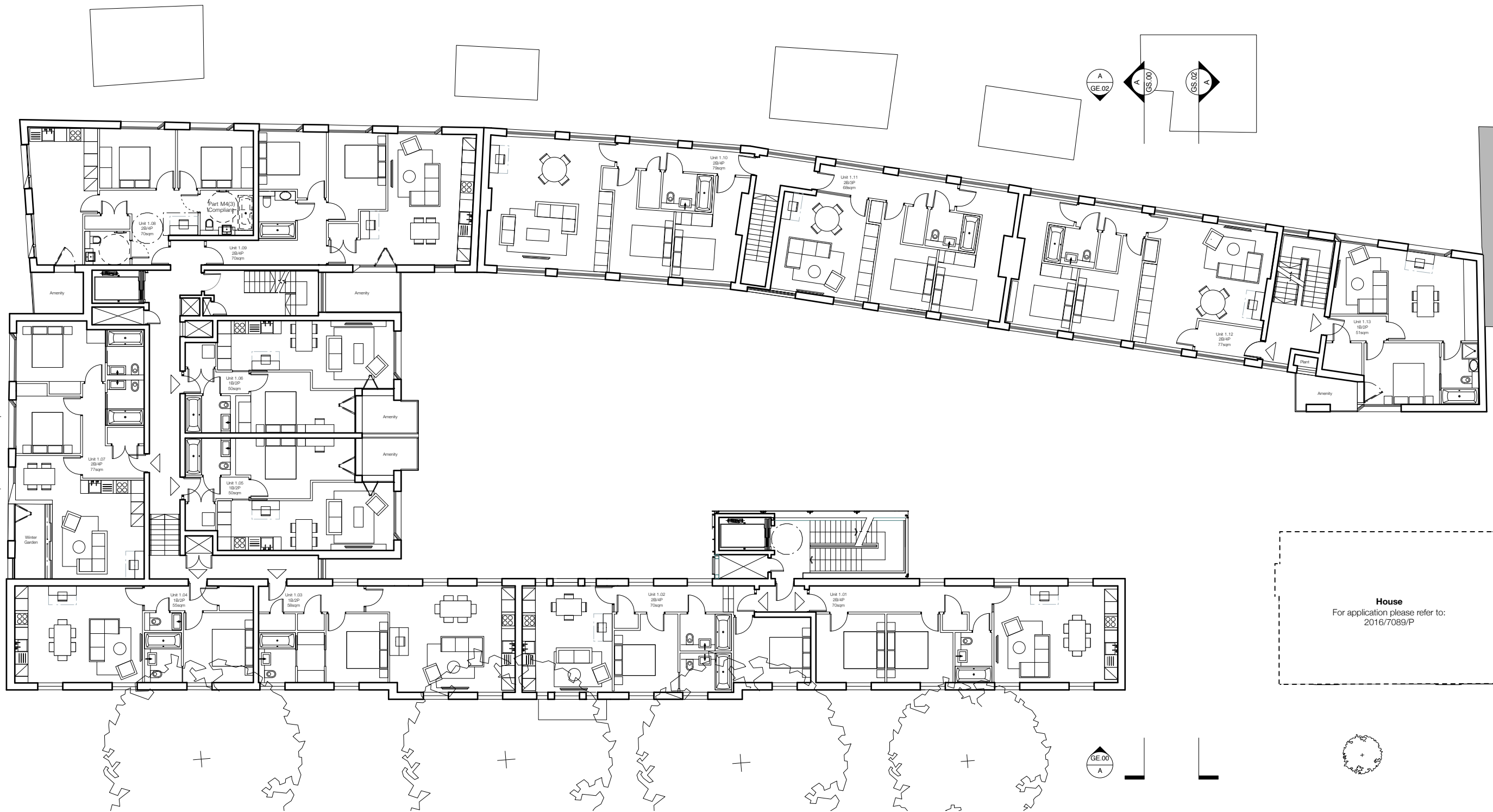
A Proposed First Floor General Arrangement GA.01 1:100 @A1 1:200 @A3
