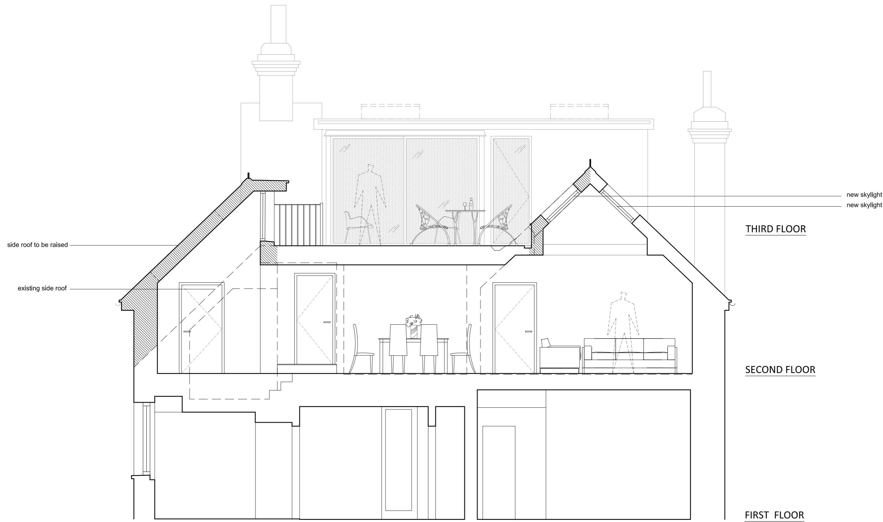
1 SECTION A 1:50@A2
