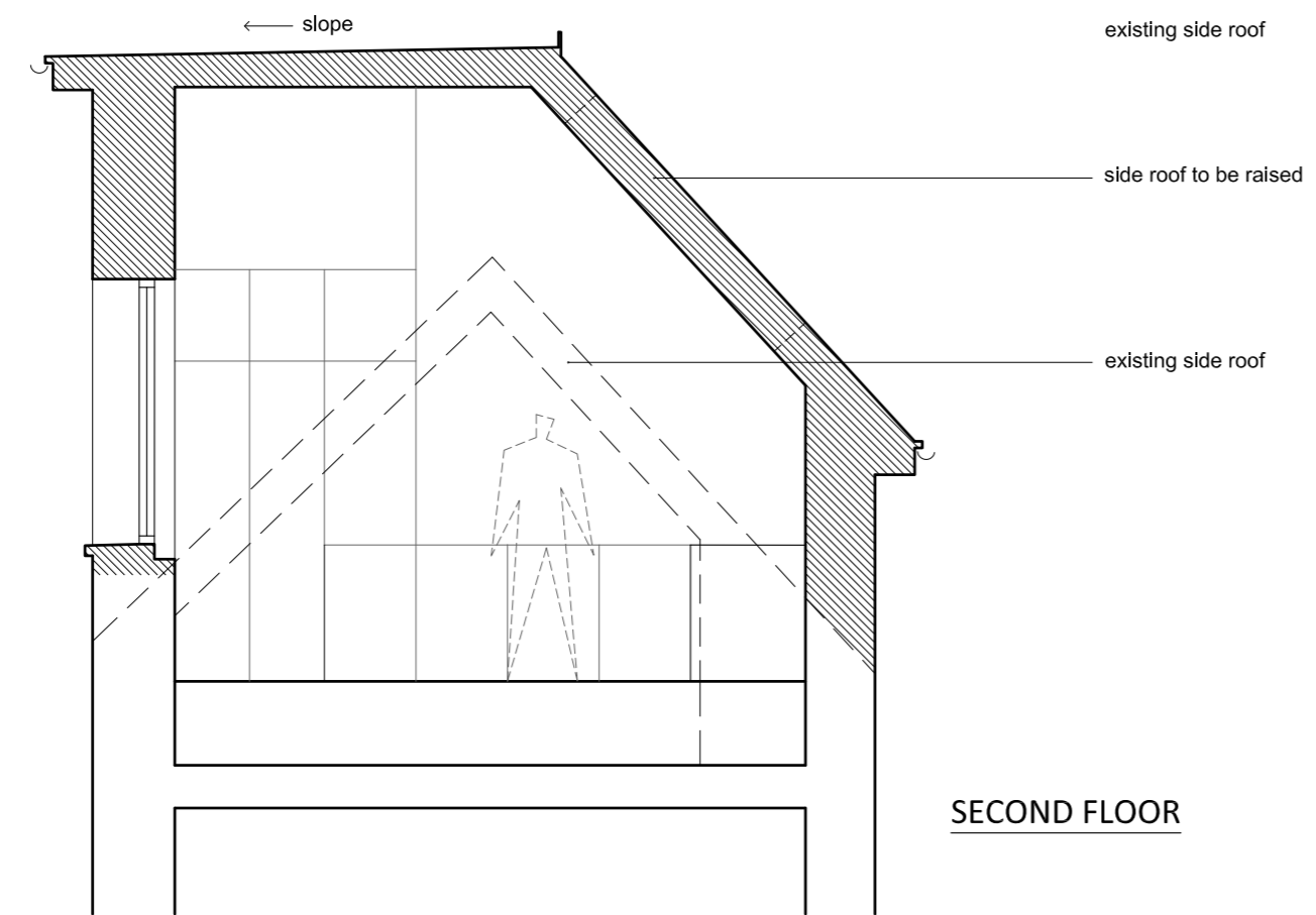
2 SECTION C 1:50@A2
