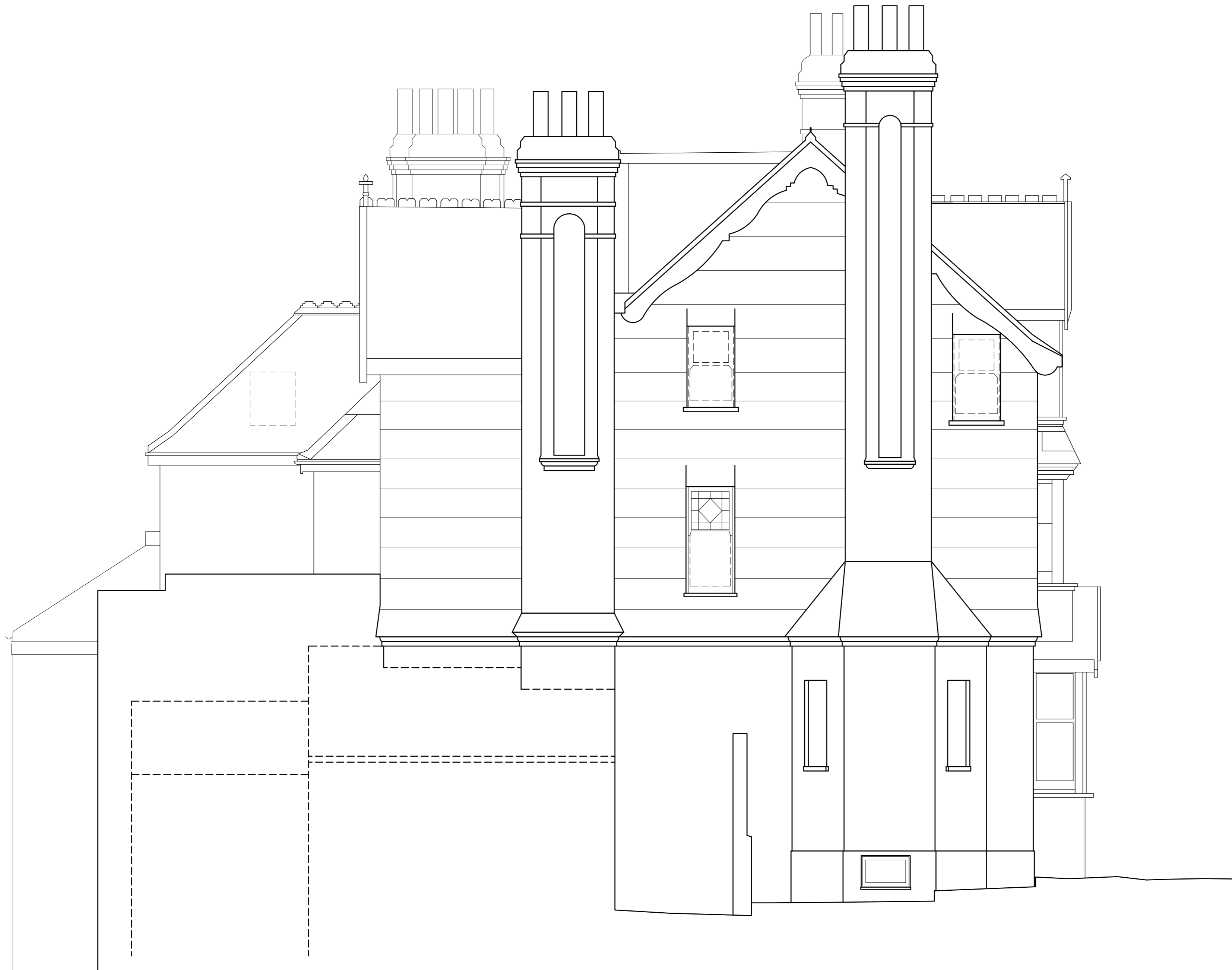
1 SIDE ELEVATION (EAST) 1:50@A2
