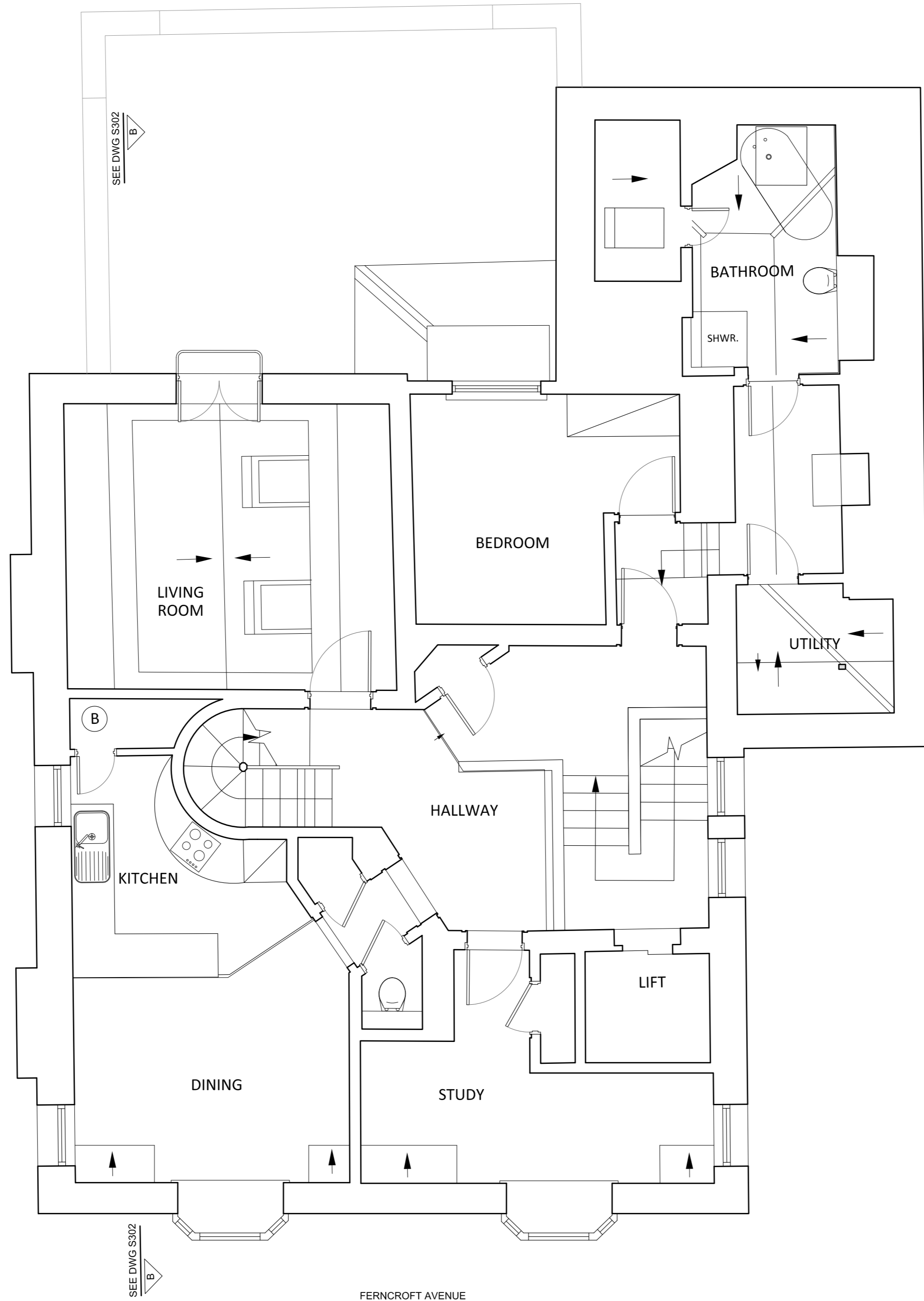
1 PROPOSED SECOND FLOOR 1:50@A2
