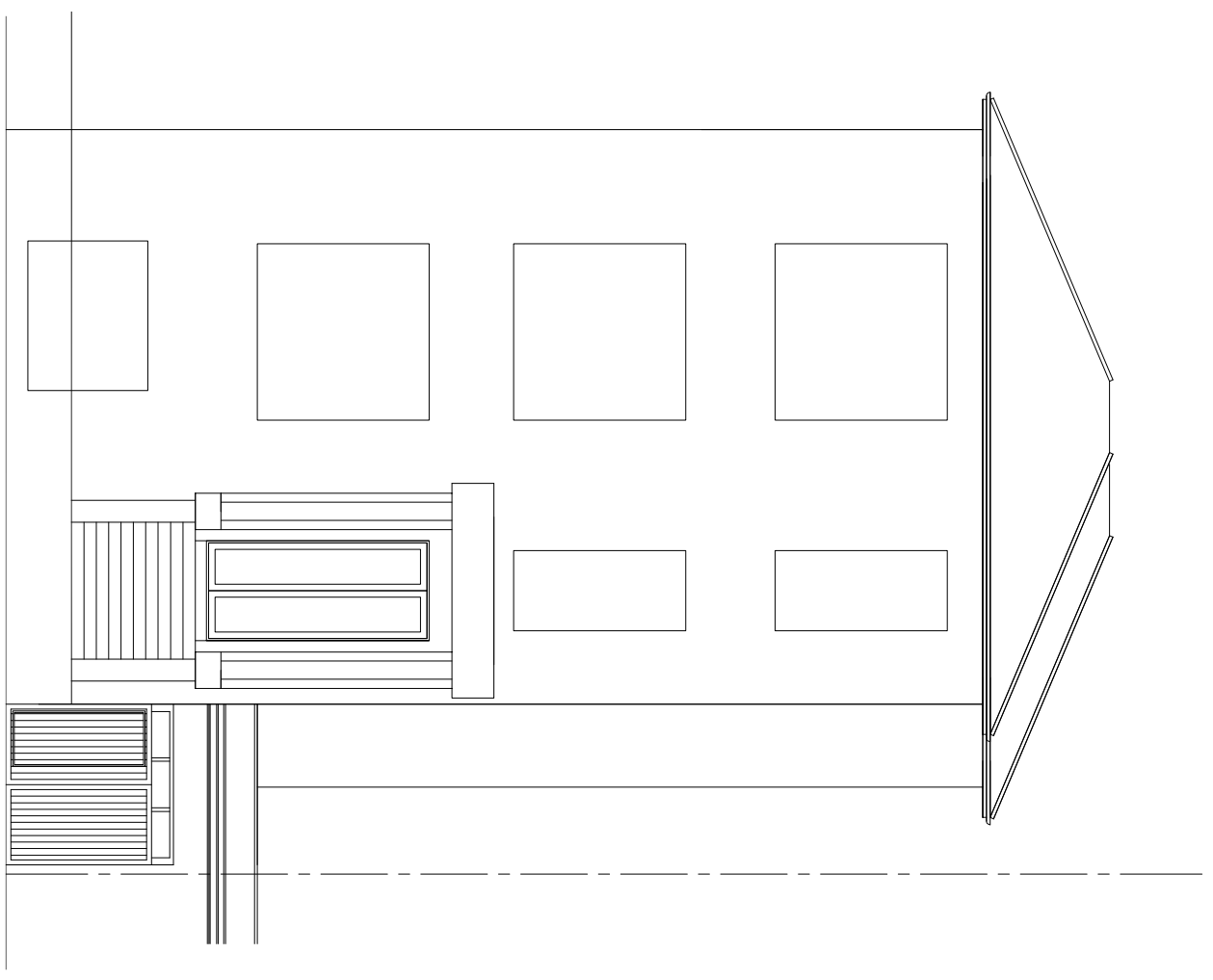
FRONT ELEVATION 1:100
