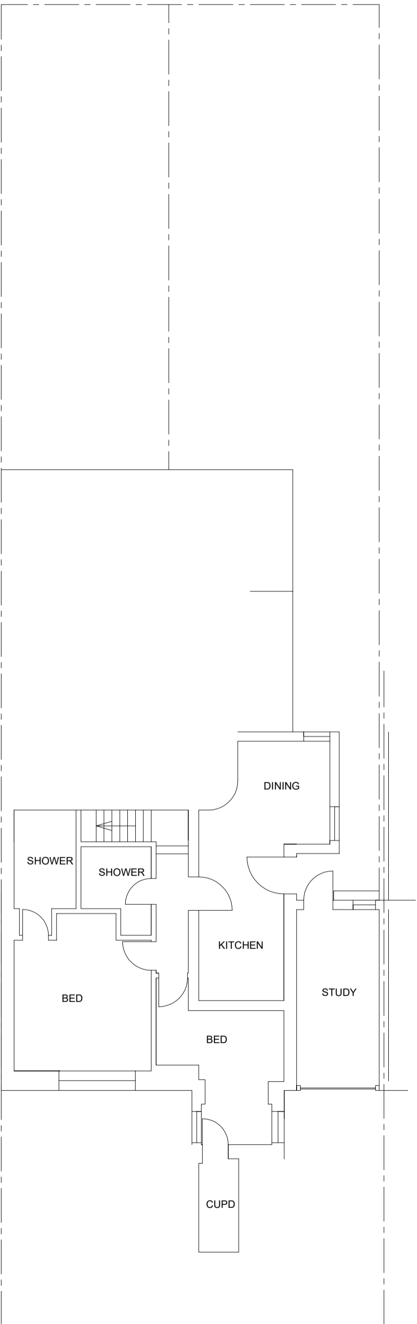
LOWER GROUND FLOOR PLAN
