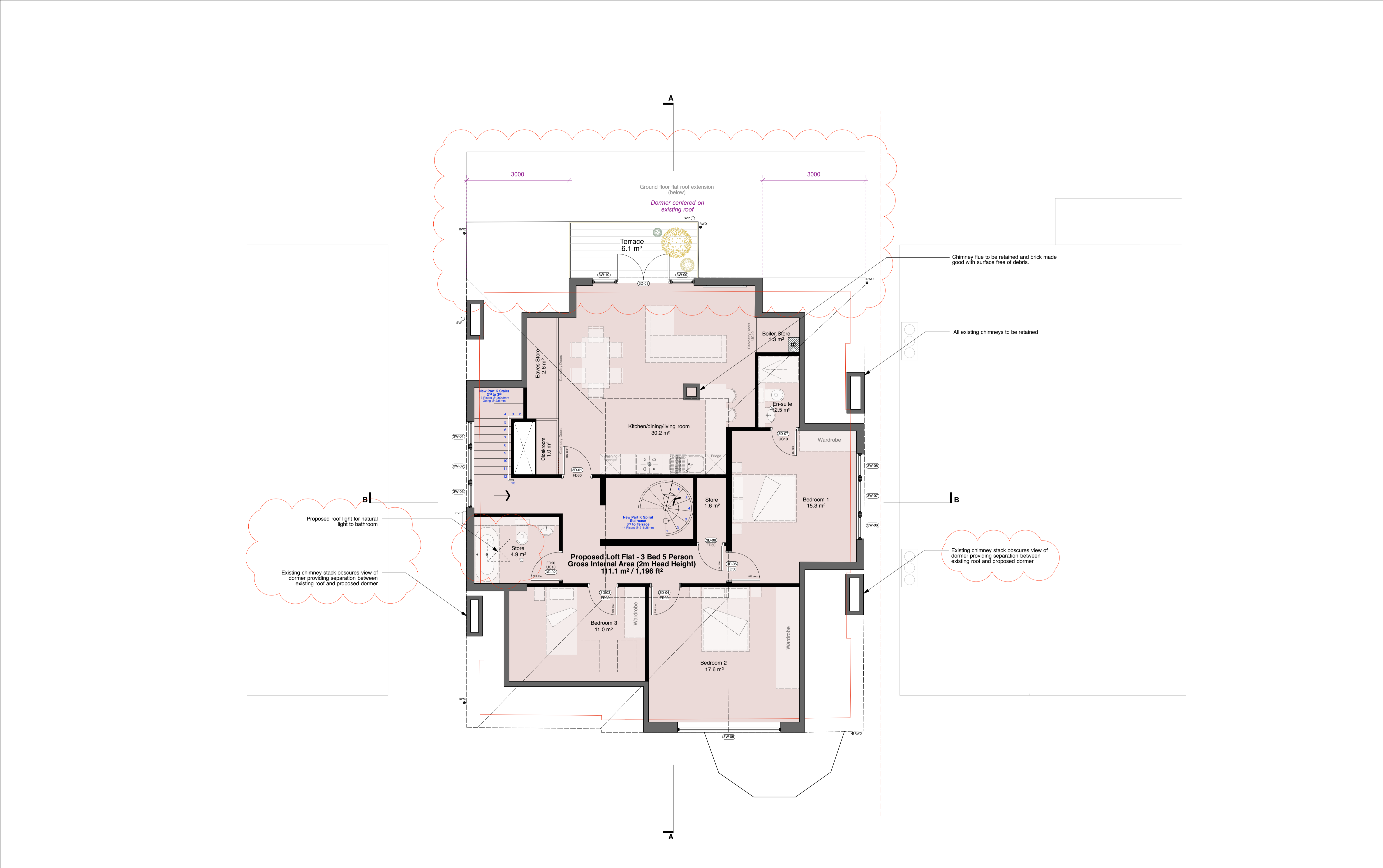
PROPOSED LOFT PLAN
