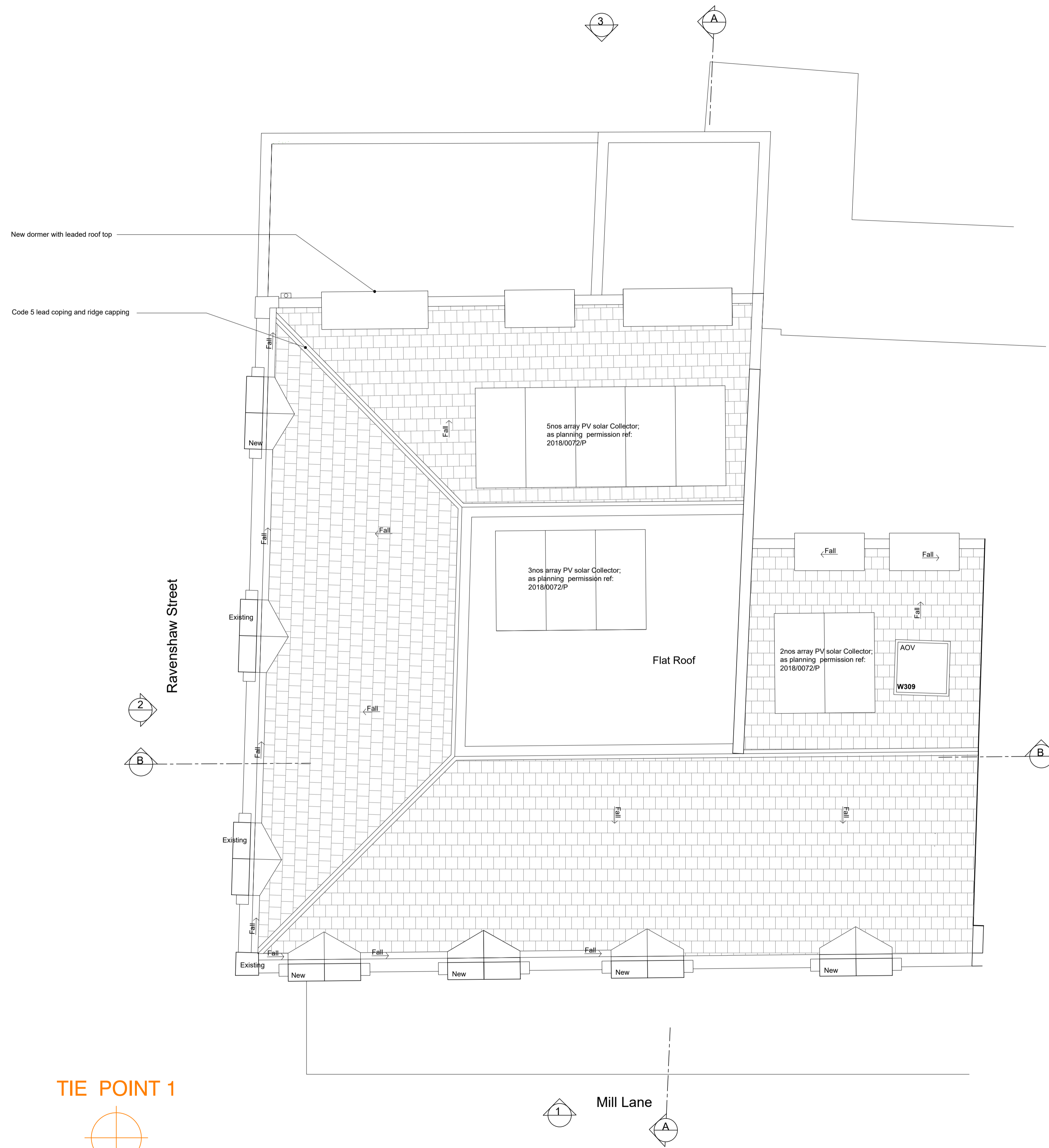
1 Existing Roof Plan (Under Construction) as approved scheme ref:2016/2661/P
