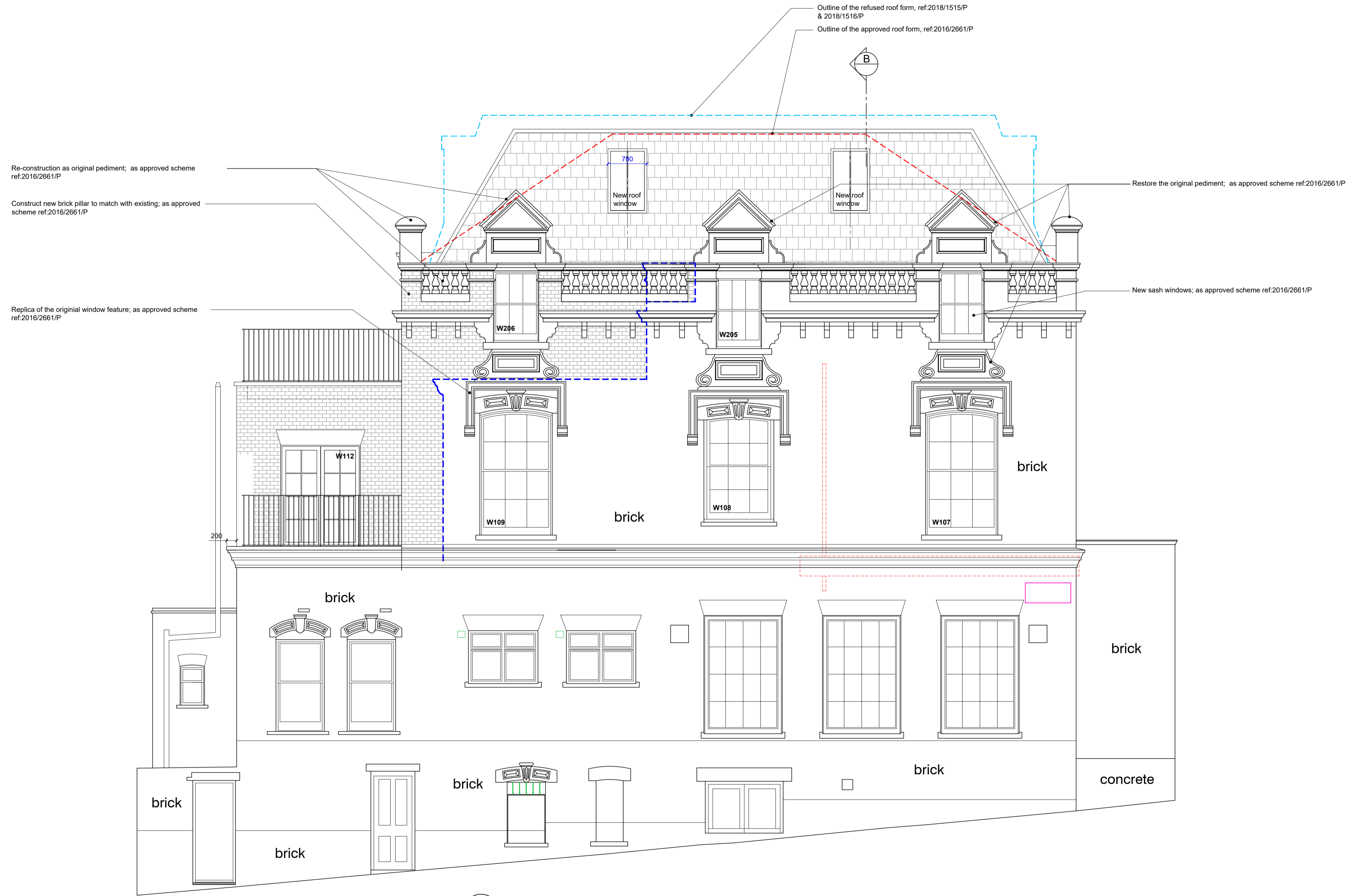
1 Proposed Elevation 2 at Ravenshaw Street
