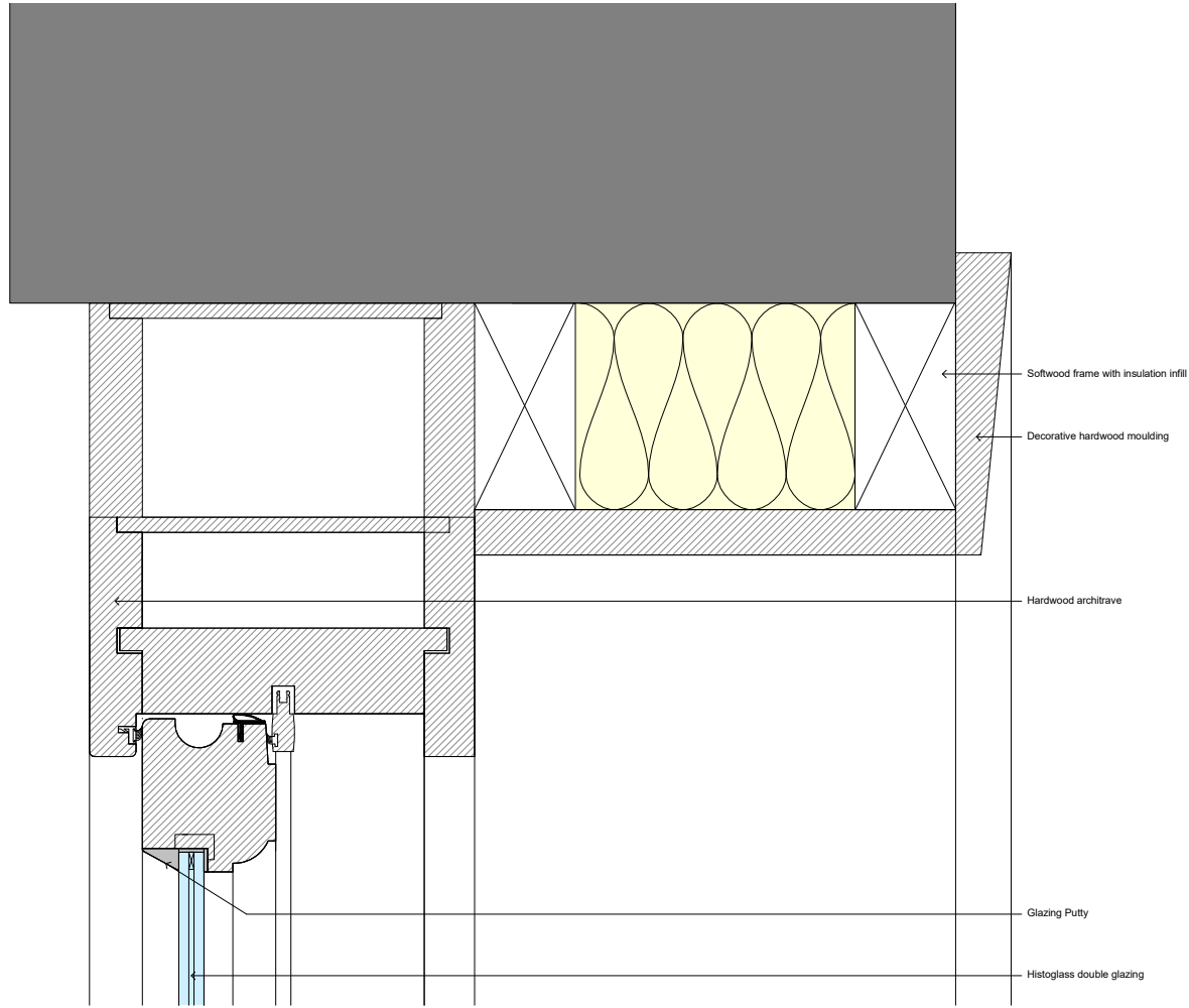
1 26 Denmark Street Typical South Architrave and Moulding Details (Window Types O, P, P1 & N) Scale: 1 : 1
