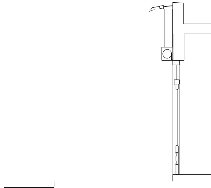
EXISTING SHOPFRONT SECTION 1:50
