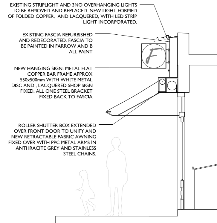
PROPOSED SHOPFRONT SECTION 1:50
