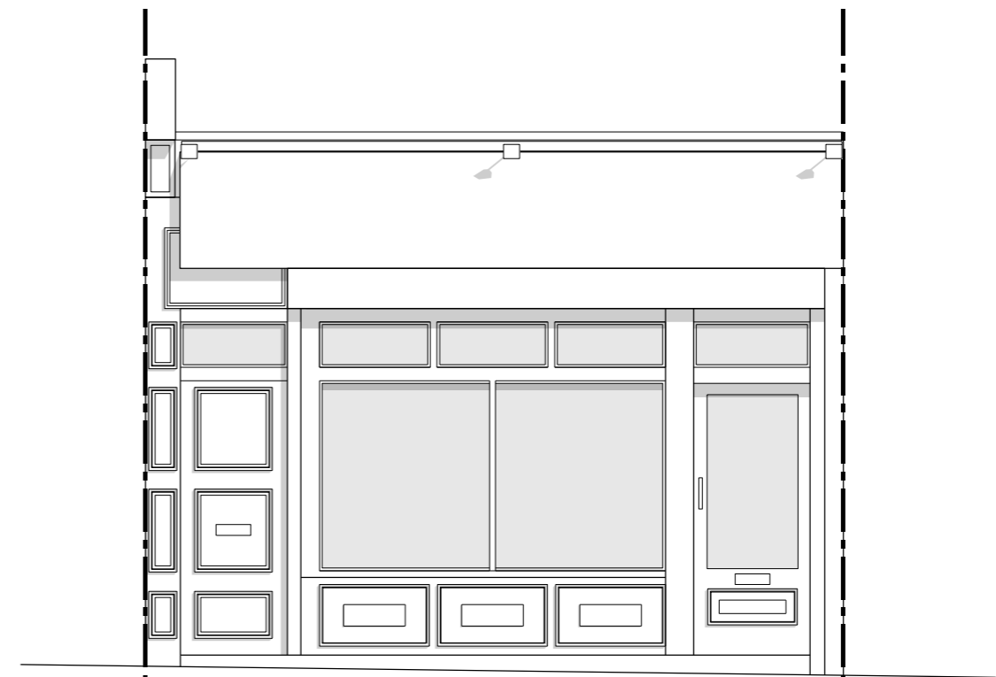
EXISTING SHOPFRONT ELEVATION 1:50
