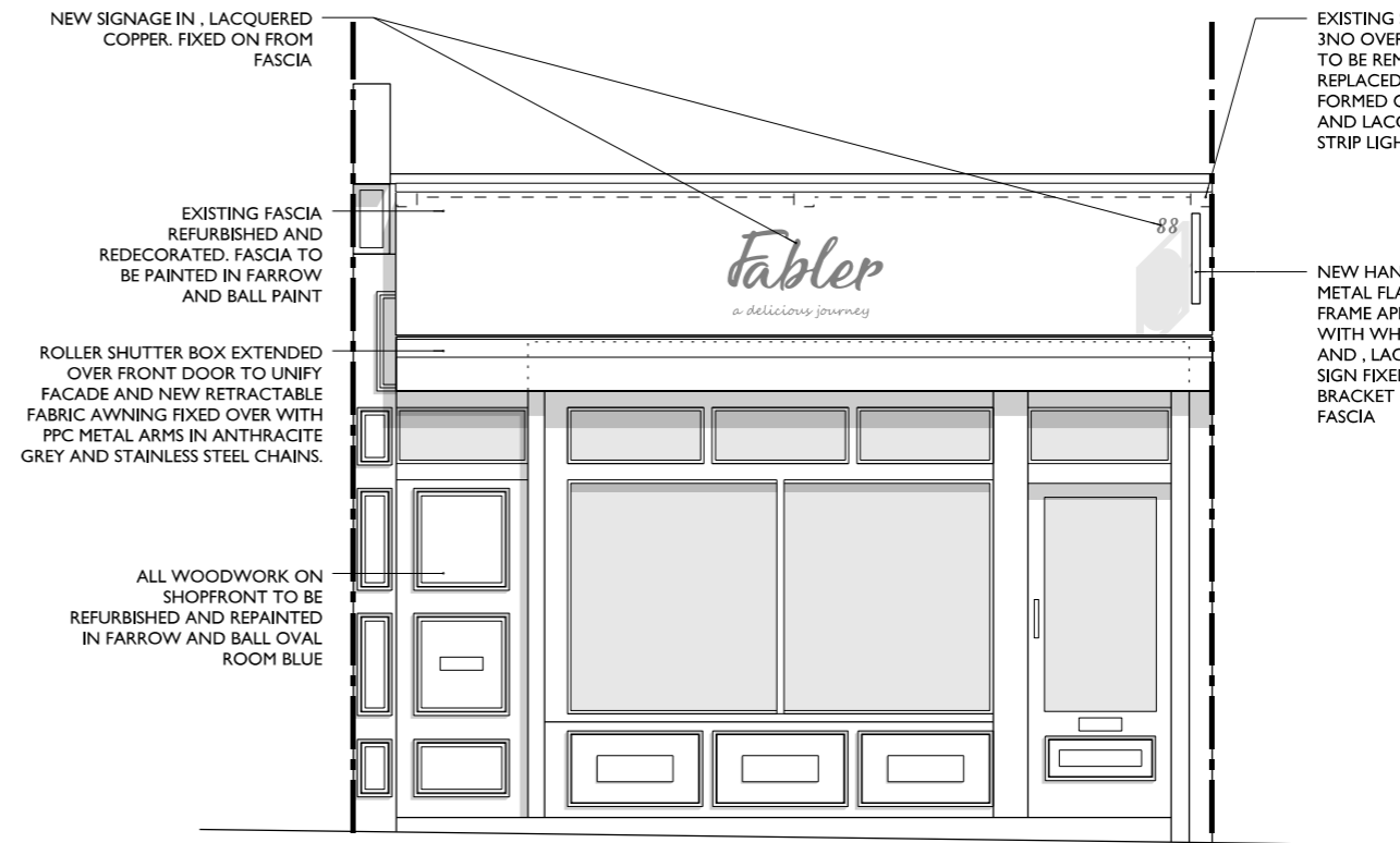
PROPOSED SHOPFRONT ELEVATION 1:50
