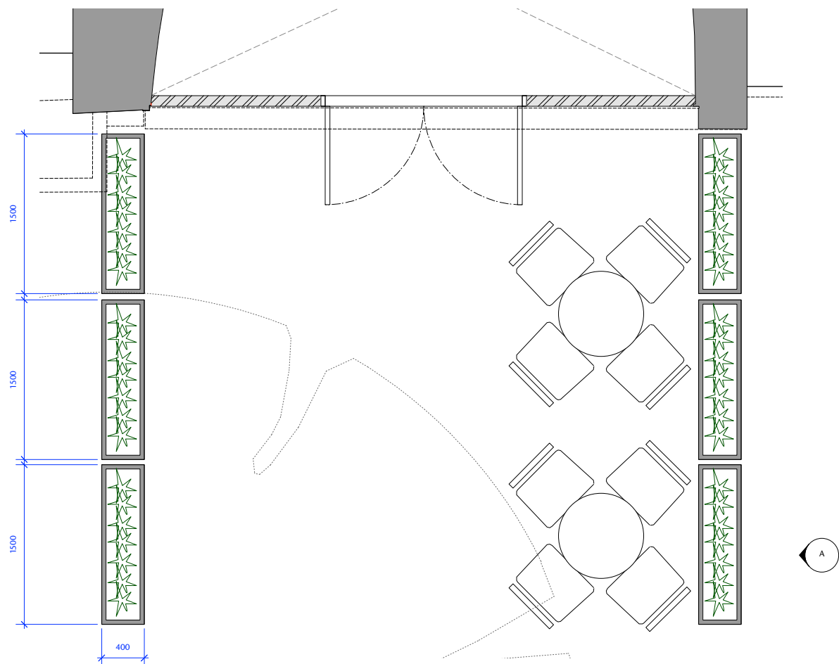
1 PLANTER PLAN 1:25 @ A1
