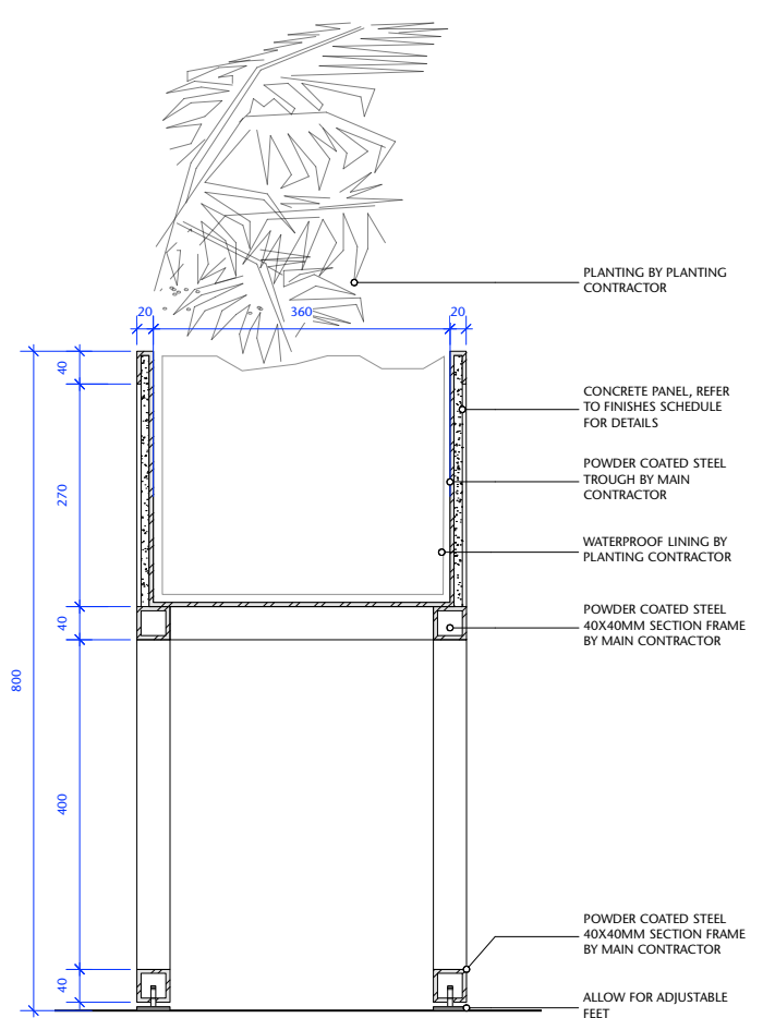
4 PLANTER SECTION CC 1:5 @ A1
