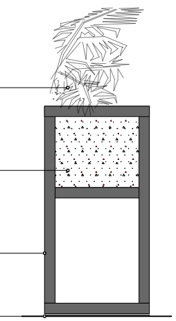
3 PLANTER ELEVATION B 1:10 @ A1
