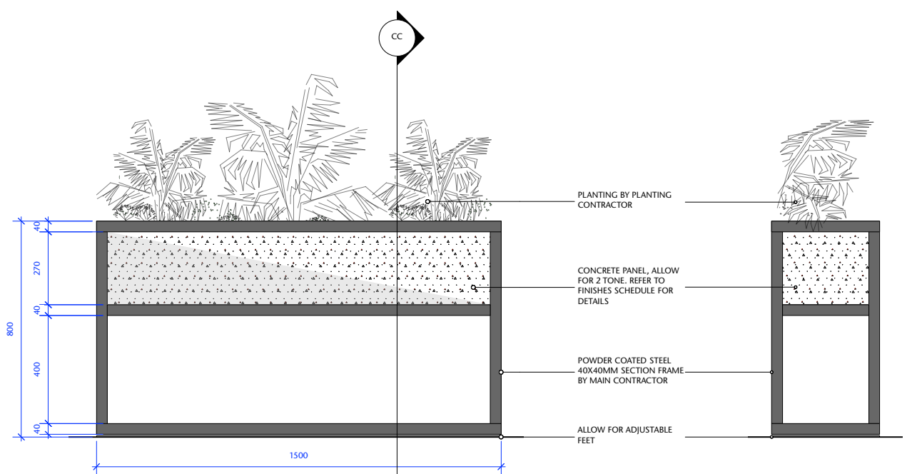
2 PLANTER ELEVATION A 1:10 @ A1
