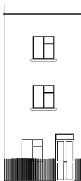
FRONT ELEVATION
