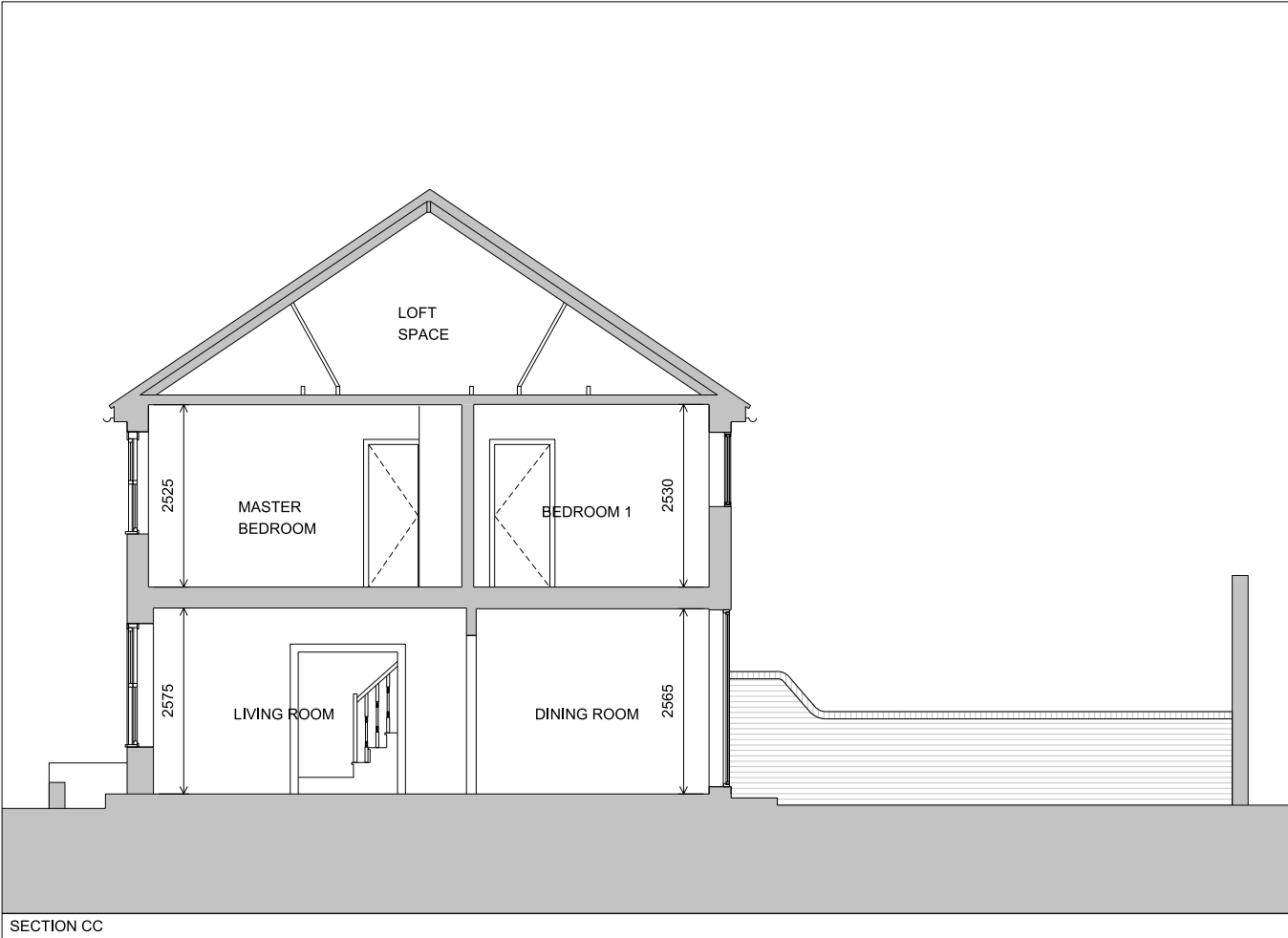
SECTION CC
