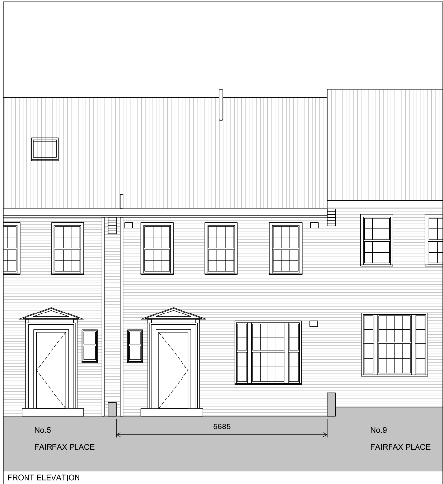
FRONT ELEVATION
