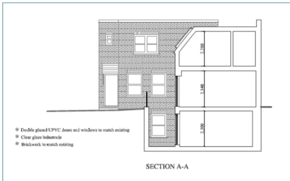
Figure 5 Proposed Section A-A
