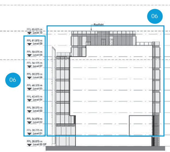
3- North Elevation Block S2
