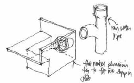
4 3D Sketch of RWP / Upstand Interface
