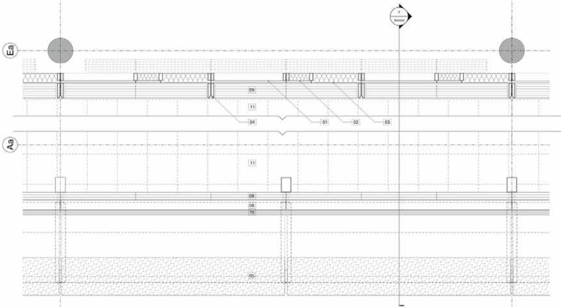
3 Plan Level 08
