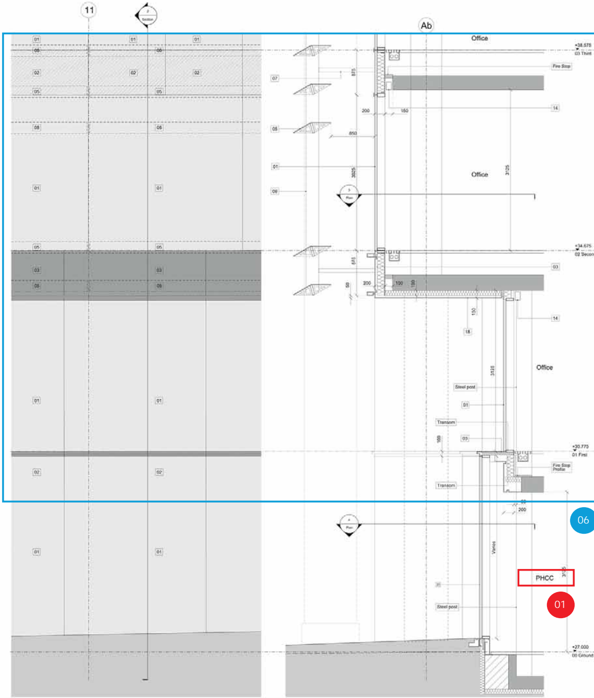
1 Elevation View
