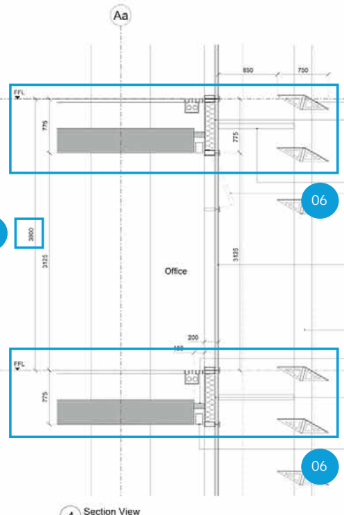
4 Section View
