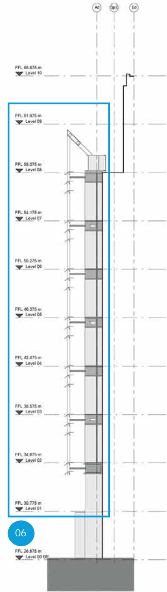
1503-20-323 - North Return Elev. N2
