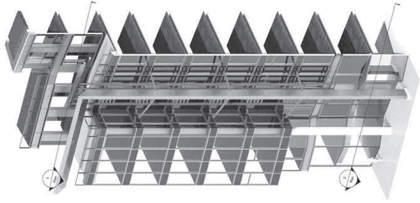
3 Axo View N1 Return (without busses for visual purposes)
