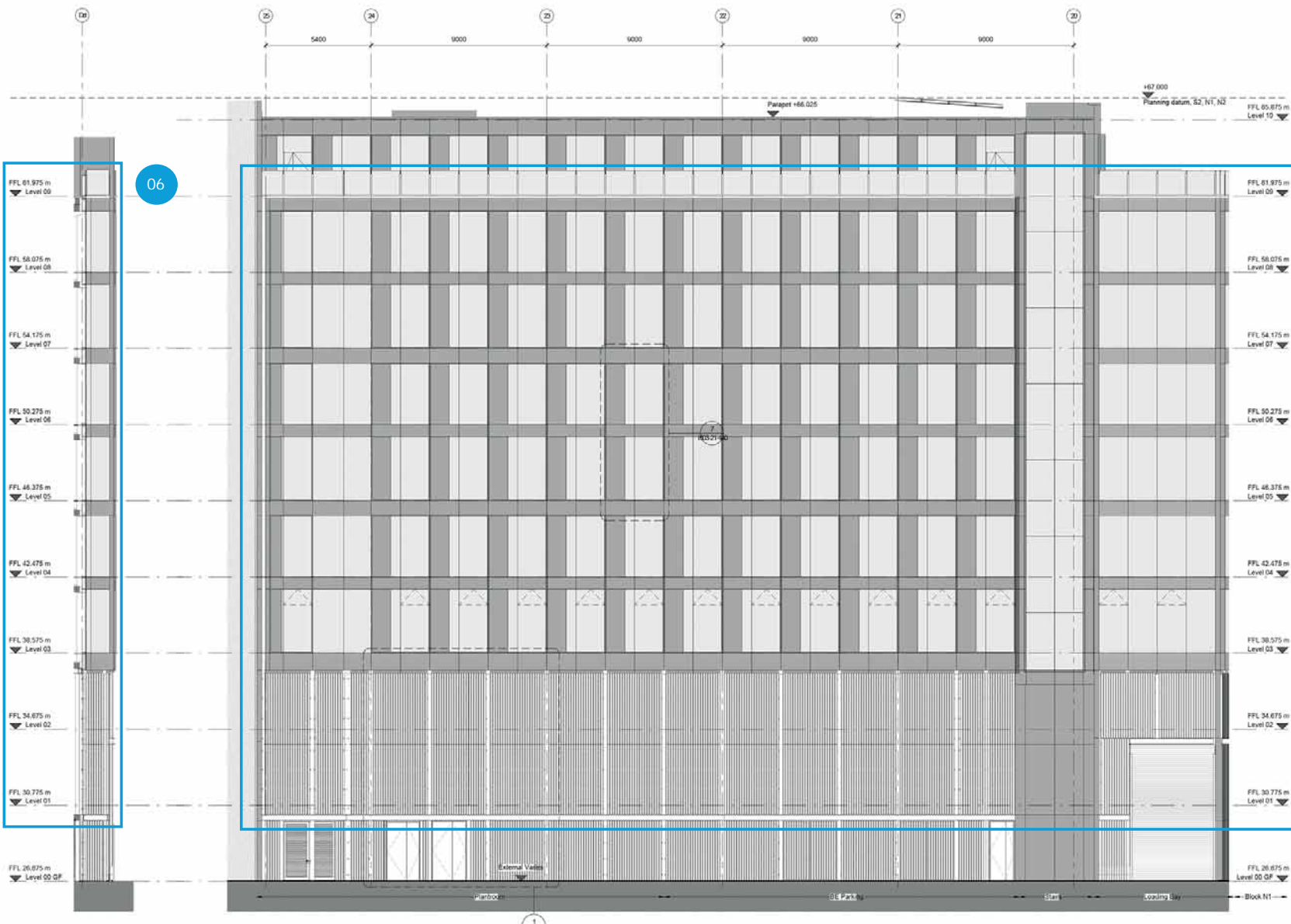
North Return Elev. N2
