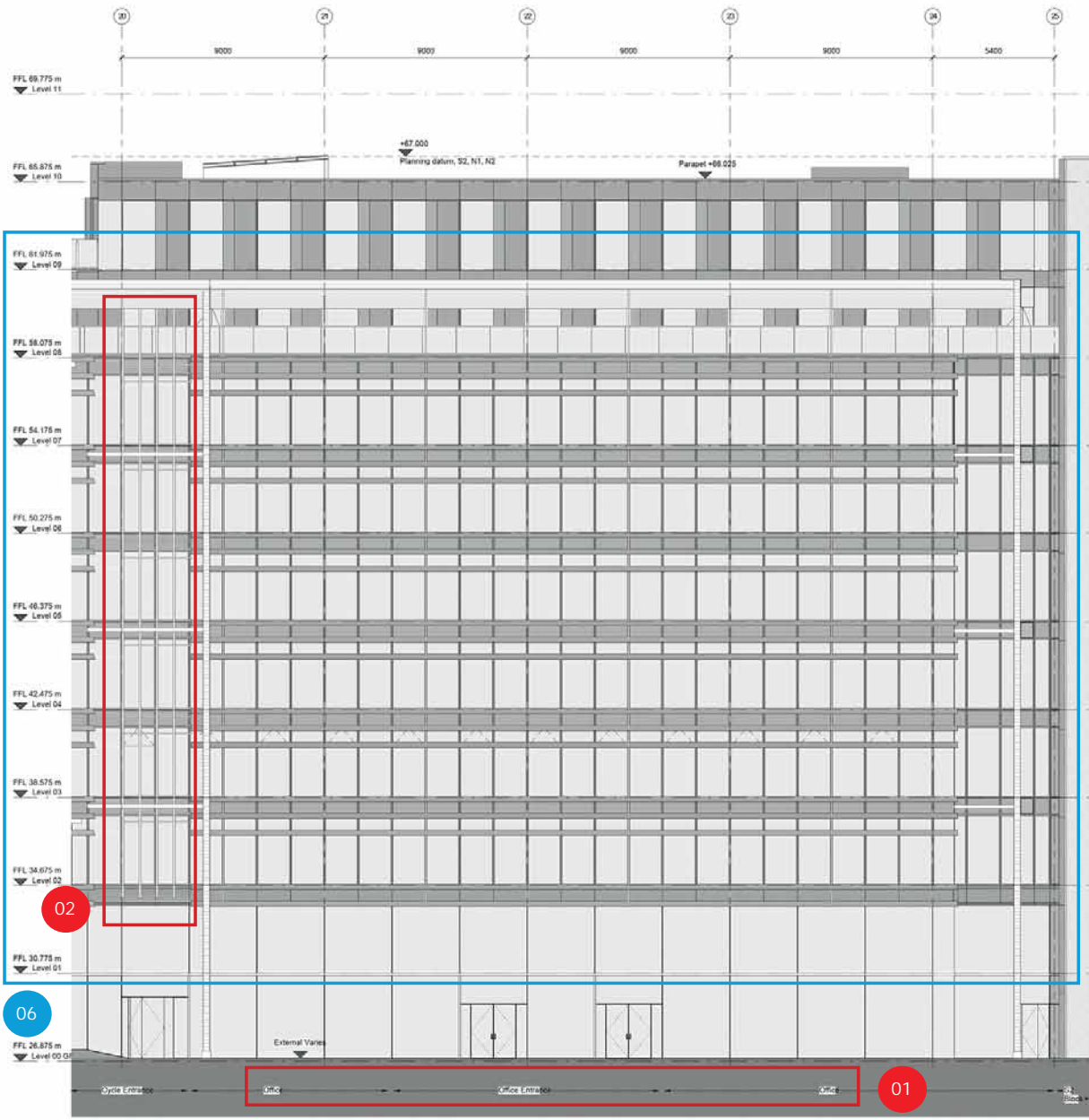
East Elevation N2
