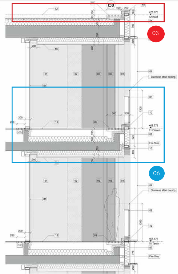
2 Section View
