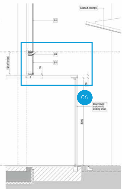
3 Section View
