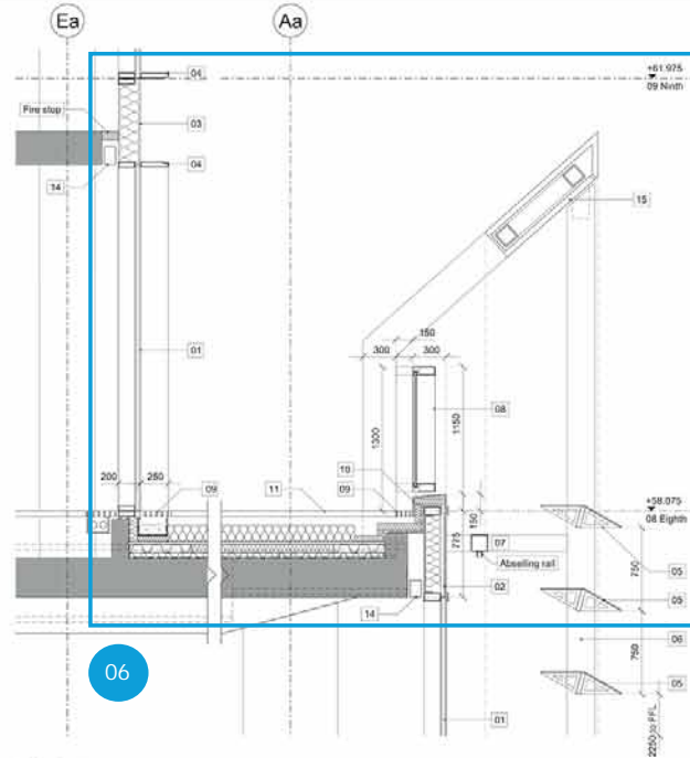
2 Section
