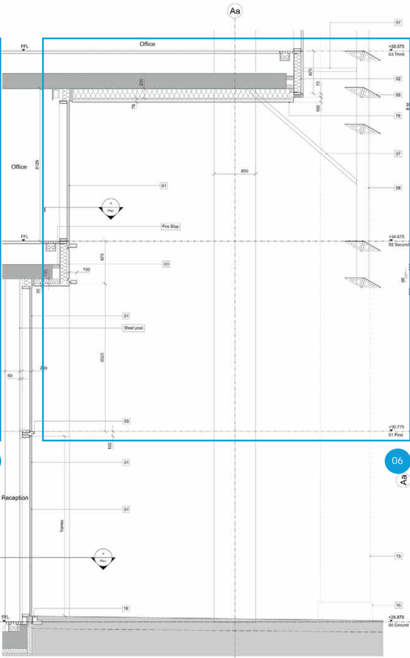
2 Section View
