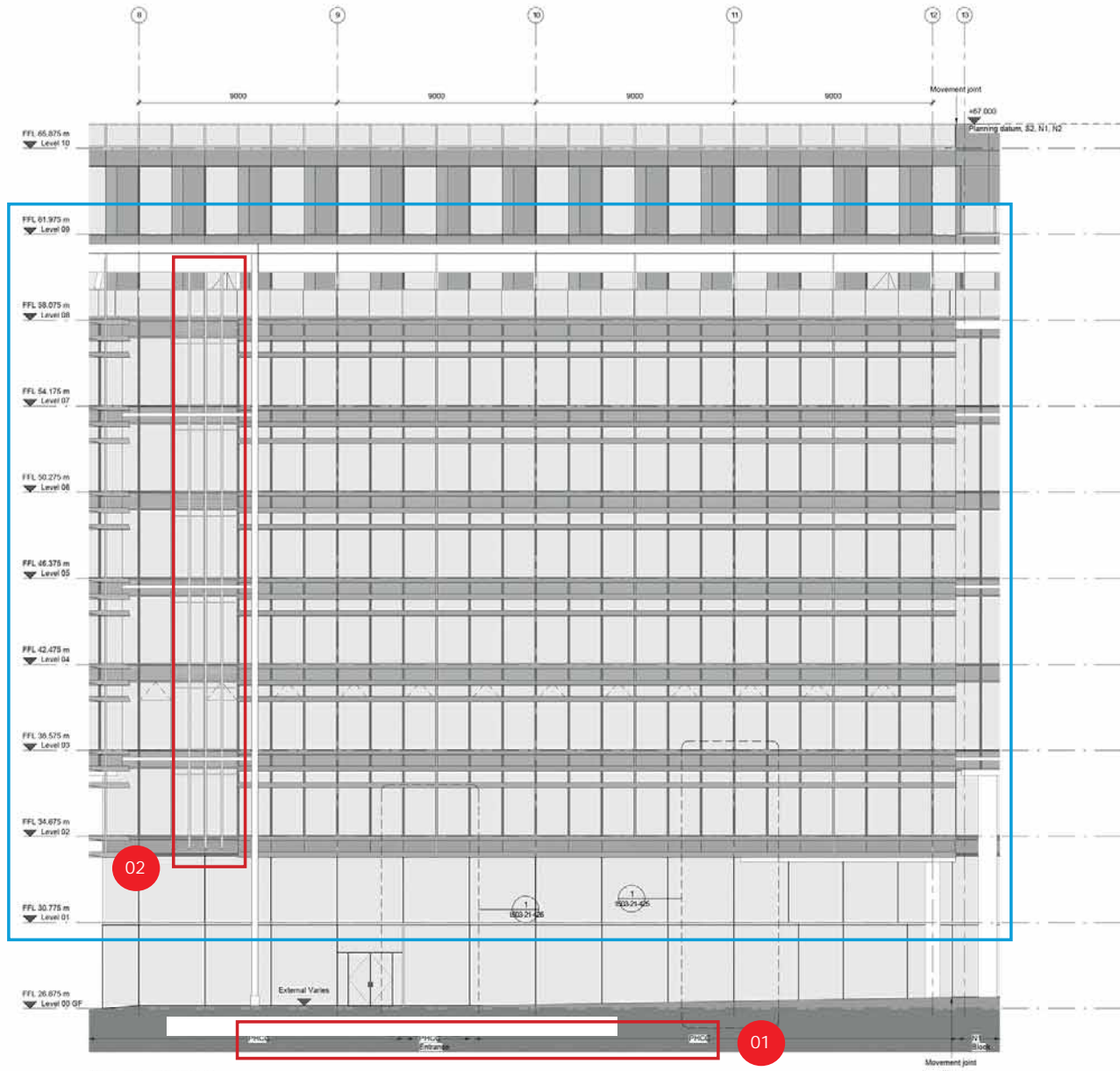
East Elevation S2
