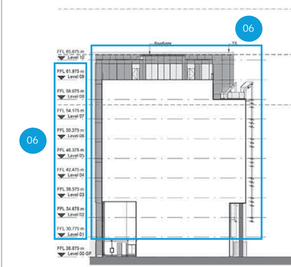
2- South Elevation N2
