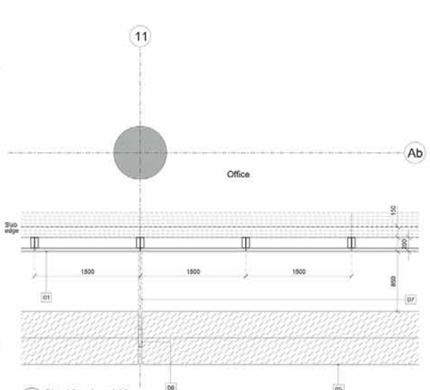
3 Plan View Level 02
