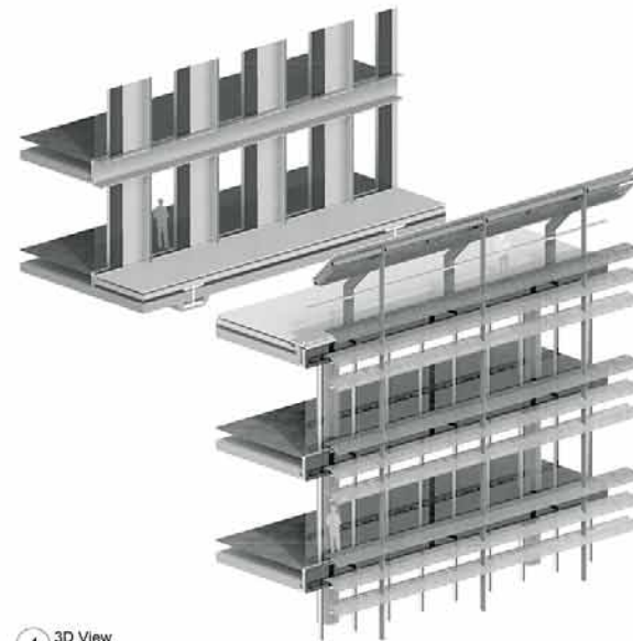
4 3D View
