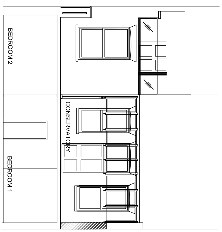
BASEMENT AND LOWER GROUND SHORT SECTION BB AS PROPOSED
