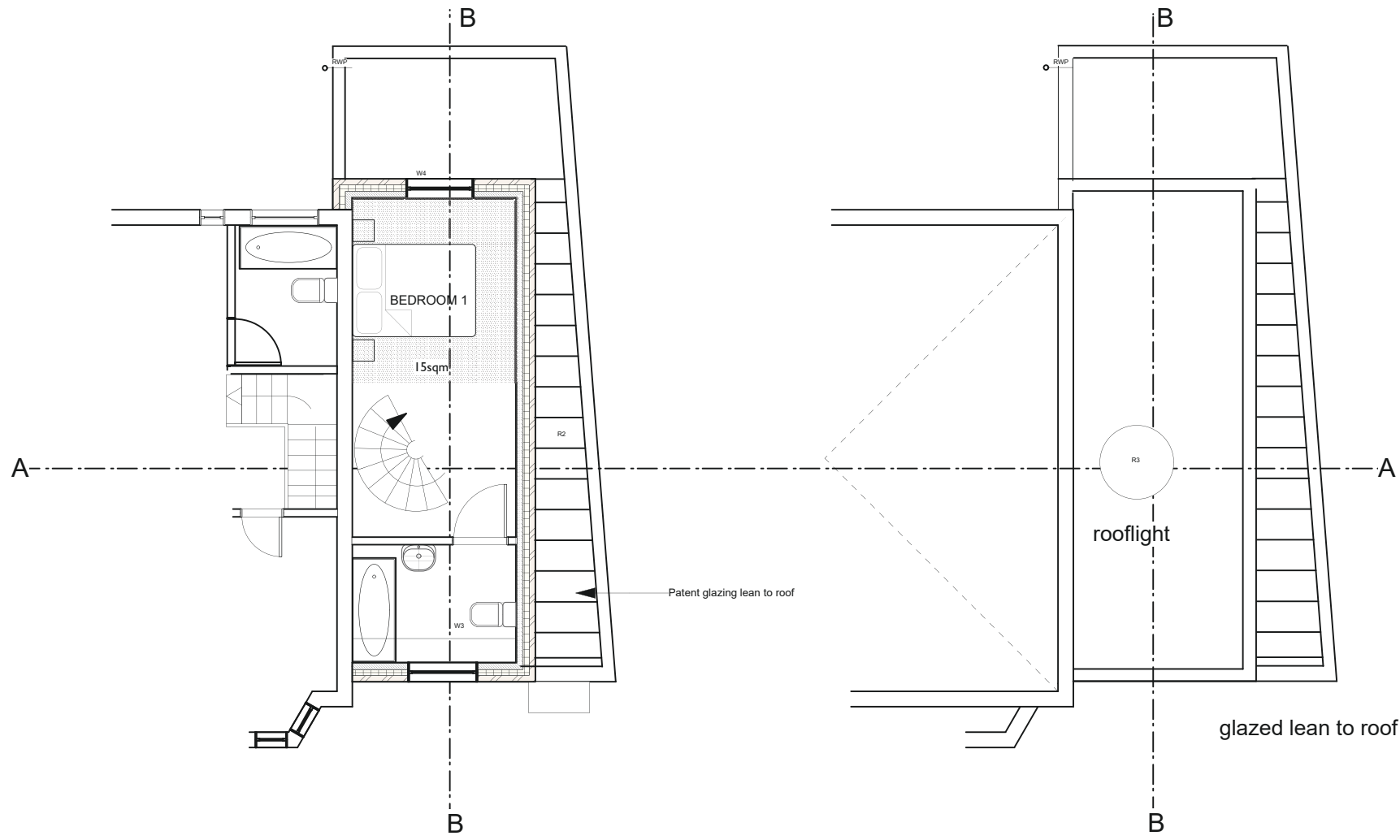
First Floor Plan as Proposed
