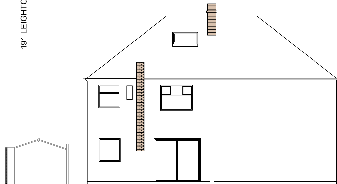
North Elevation (Garden) as Existing
