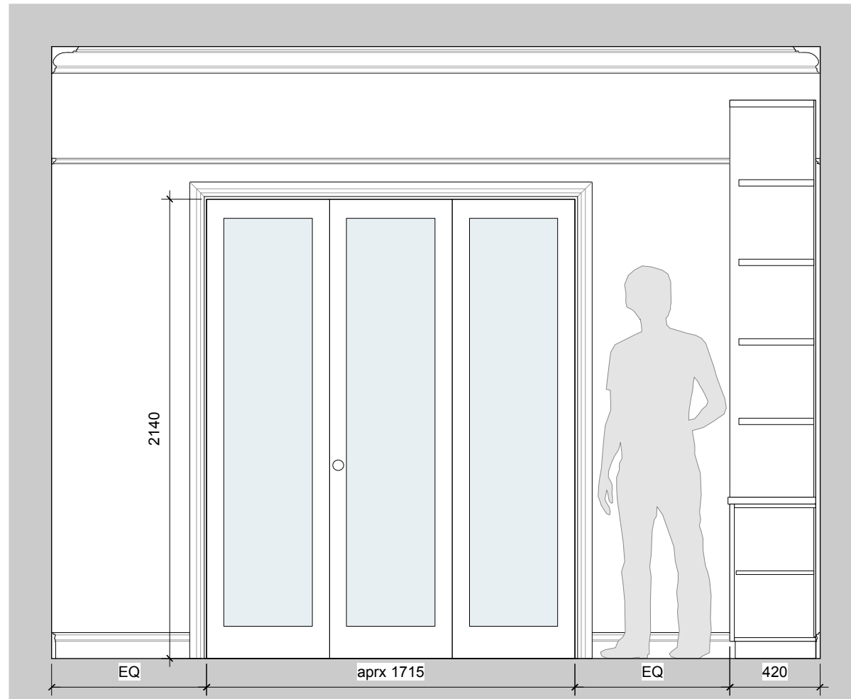
Proposed Internal Glazed Bifold Doors G3 Living Room Elevation
