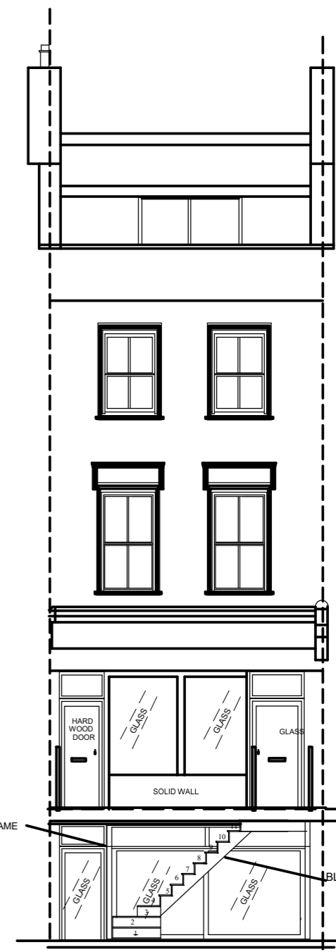
PROPOSED SECTION VIEW 2-2
