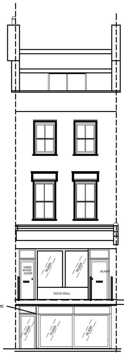
PROPOSED SECTION VIEW 1-1
