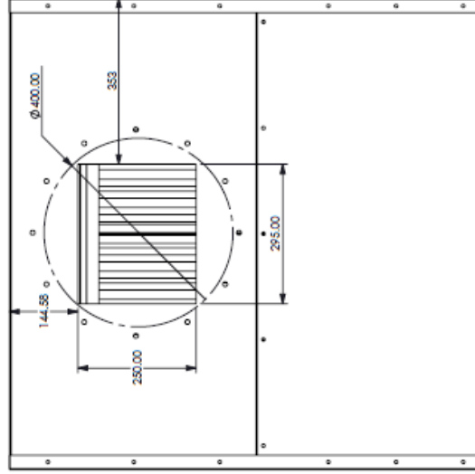
TOP VIEW OF CANOPY
