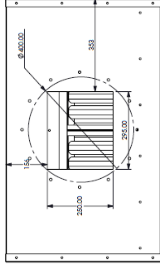
REAR VIEW OF CANOPY
